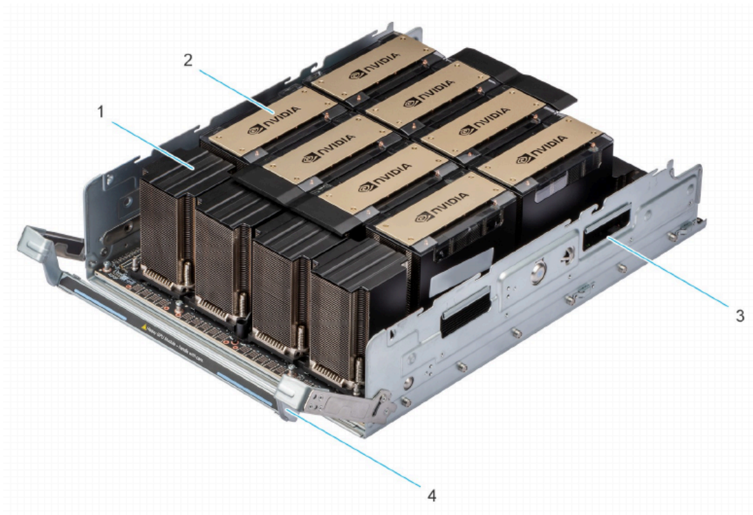
Figure 8. GPU H100/H800 Inside view
