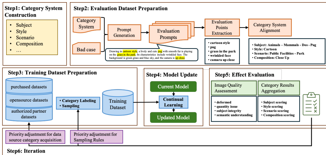
Figure 21: Illustration of our 'data convey' mechanism.
