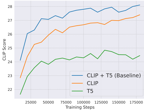
(a) CLIP Score
