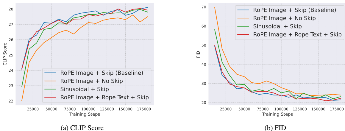
Figure 15: Ablation study on position encoding and model structure.
