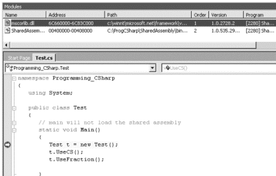
Figure 17-6. Only two modules loaded
