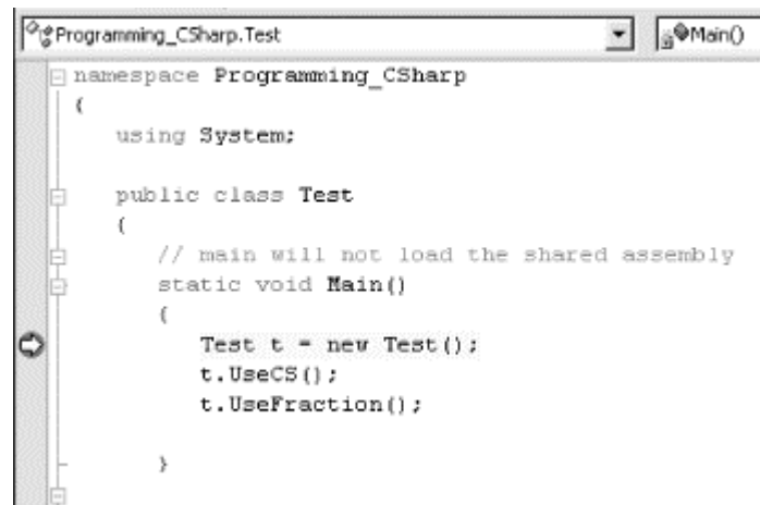
Figure 17-5. A break point in Main( )
