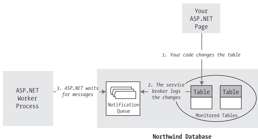
Figure 23-9. Monitoring a database for changes in SQL Server
