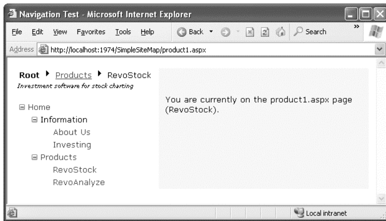
Figure 13-9. A SiteMapPath with templates
