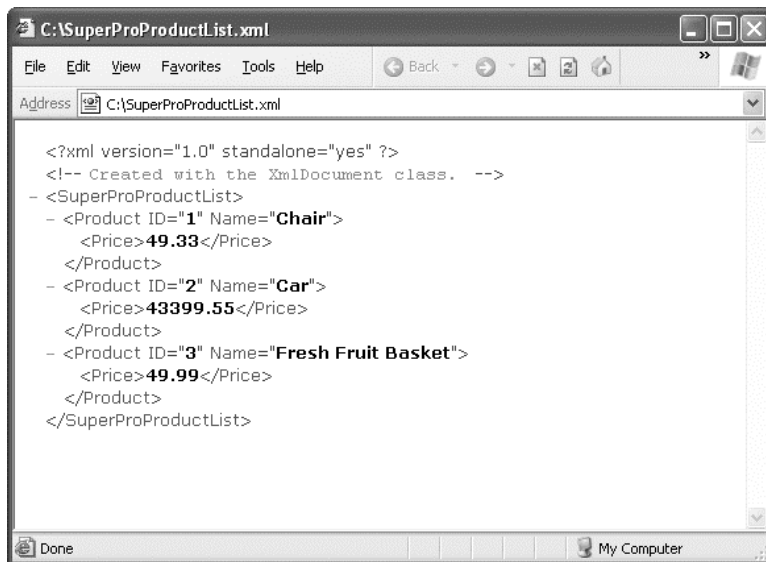
Figure 18-5. The XML file
