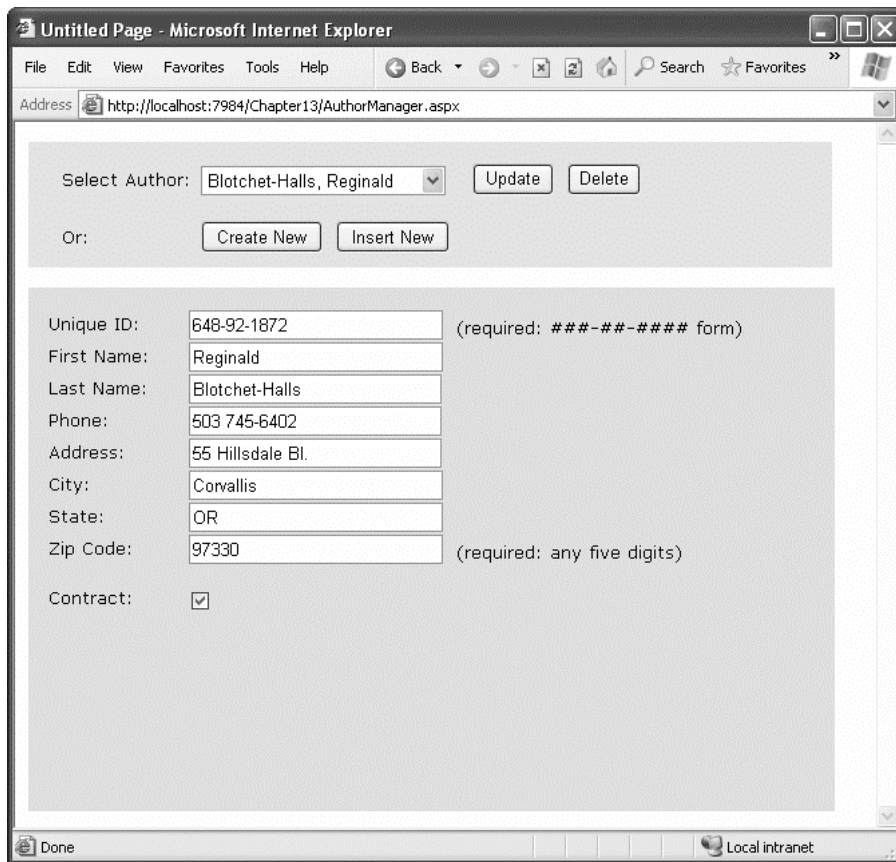
Figure 14-12. A more advanced author manager
