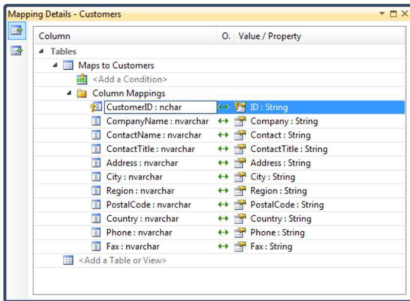
Figure 24-7. Renamed fields in the Table Mapping window
