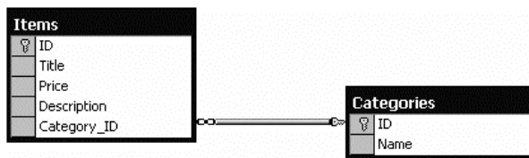
Figure 22-8. The AdBoard database relationships
