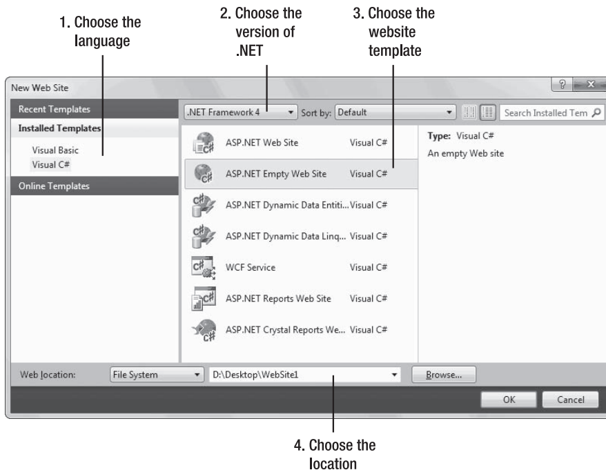
Figure 4-2. The New Web Site dialog box
