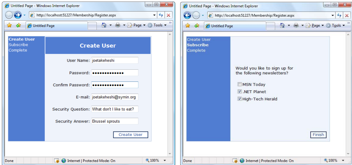
Figure 20-9. A CreateUserWizard with a custom step
