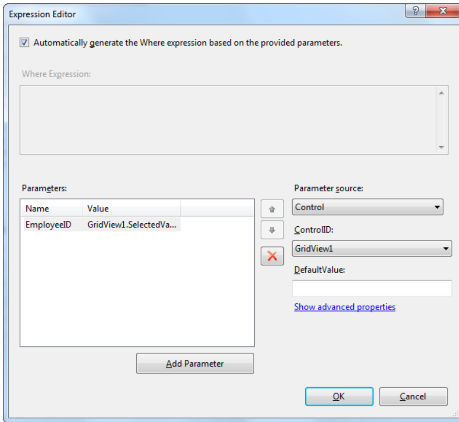
Figure 24-16. Filtering out a single employee
