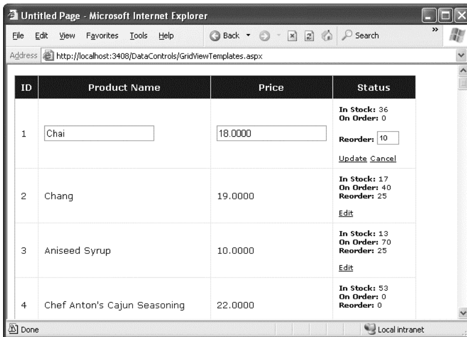
Figure 16-16. Custom edit controls
