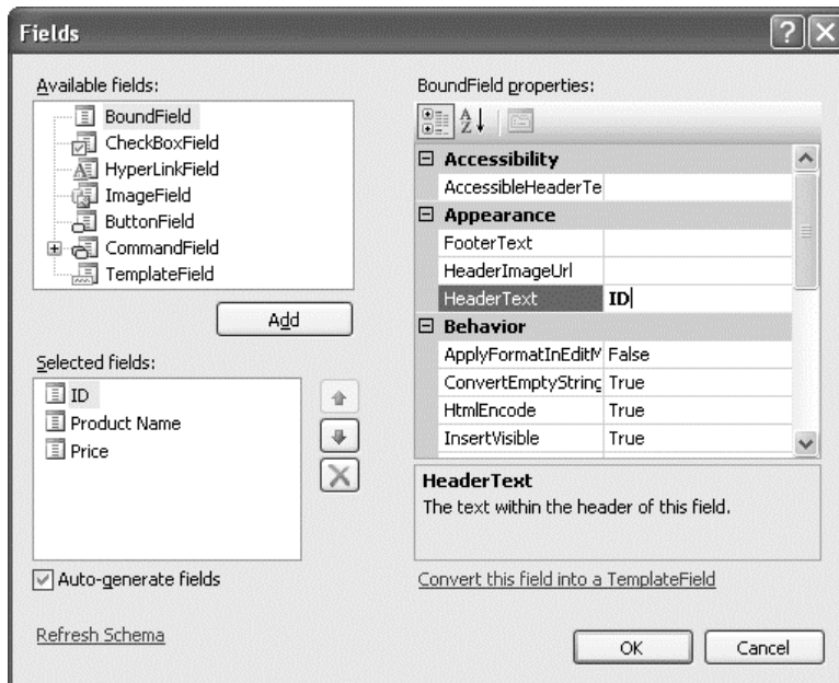
Figure 16-2. Configuring columns in Visual Studio
