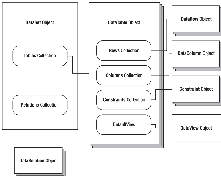
Figure 14-15. The DataSet family of objects
