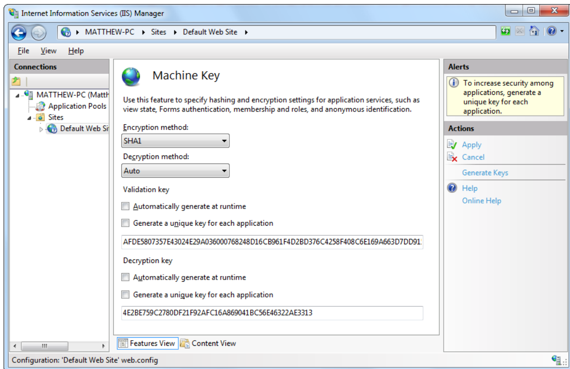
Figure 26-15. Entering fixed keys
