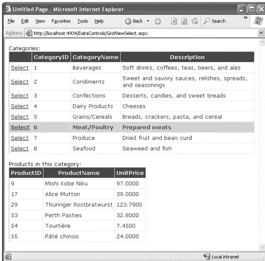
Figure 16-7. A master-details page
