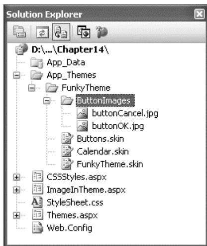
Figure 12-13. Adding images to a theme
