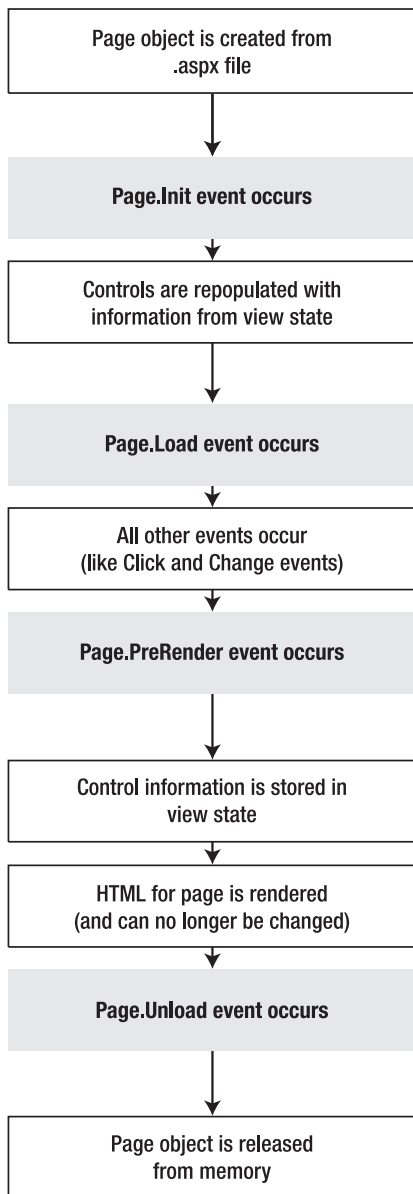
Figure 6-12. The postback processing sequence
