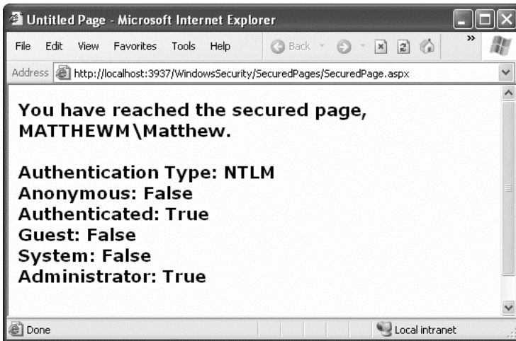
Figure 19-7. Retrieving Windows authentication information
