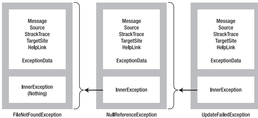
Figure 7-3. Exceptions can be chained together.
