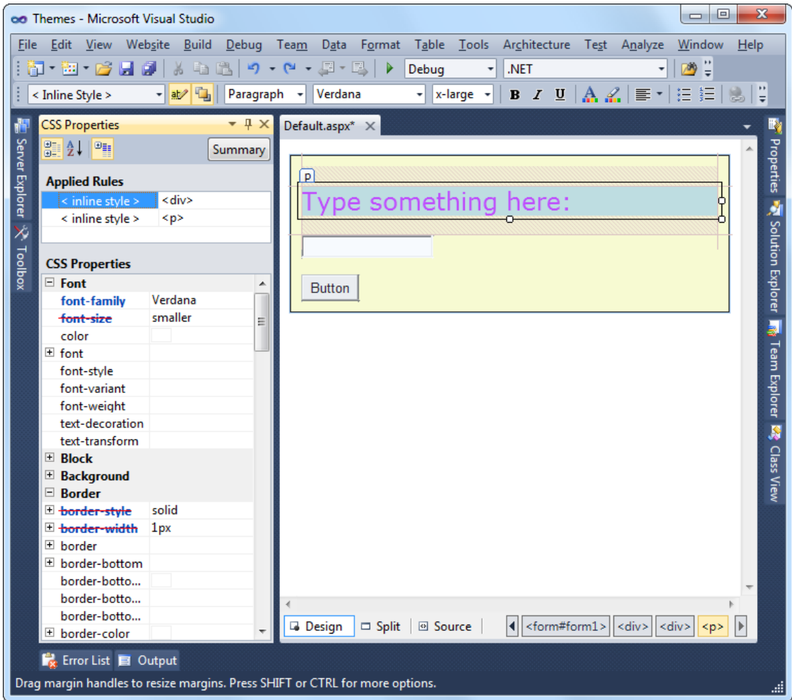
Figure 12-6. Inherited and overridden style properties
