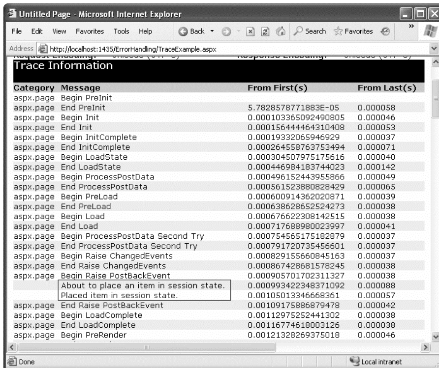
Figure 7-22. Custom trace messages
