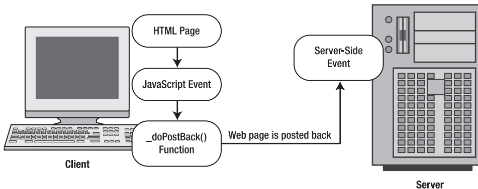
Figure 6-13. An automatic postback
