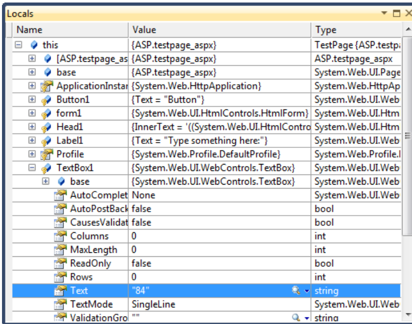
Figure 4-25. Viewing the current page object in the Locals window
