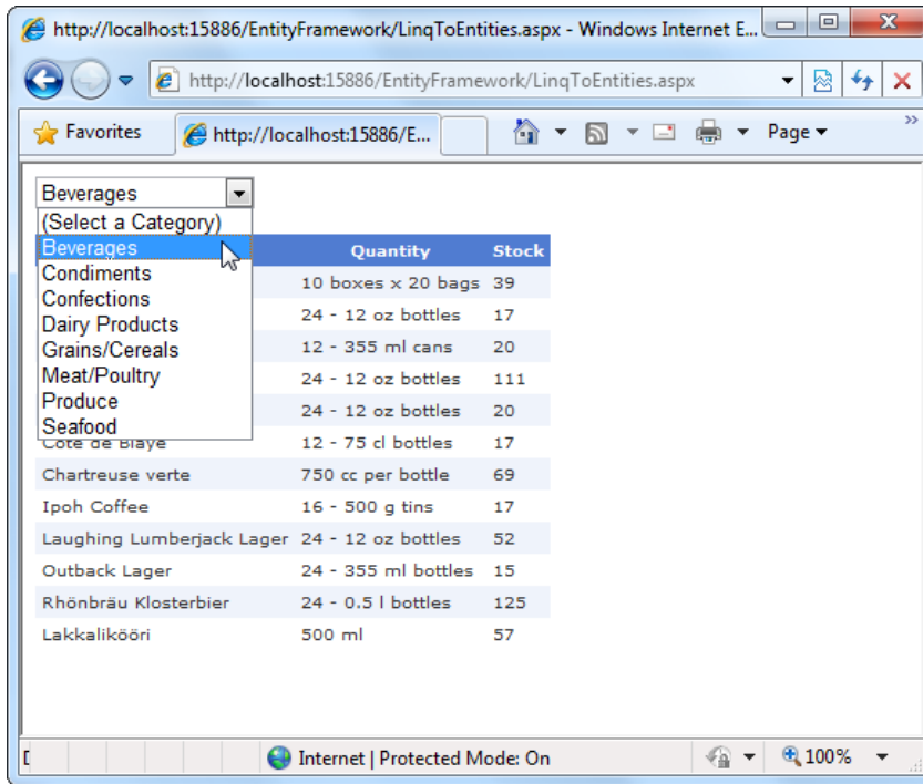
Figure 24-12. Browsing product categories
