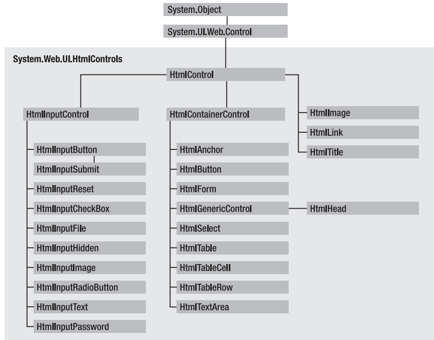
Figure 5-7. HTML control inheritance
