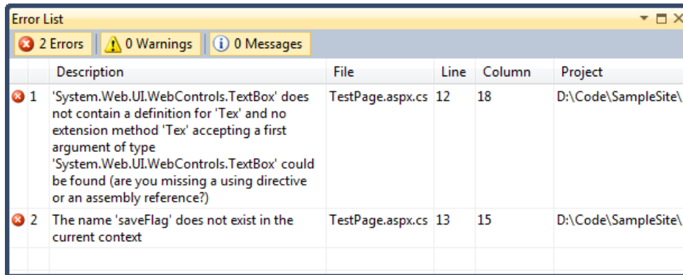
Figure 4-18. The Error List window
