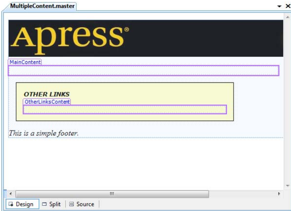
Figure 12-19. A master page with two content regions
