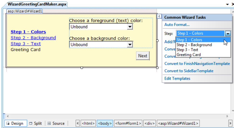
Figure 10-10. Designing a step
