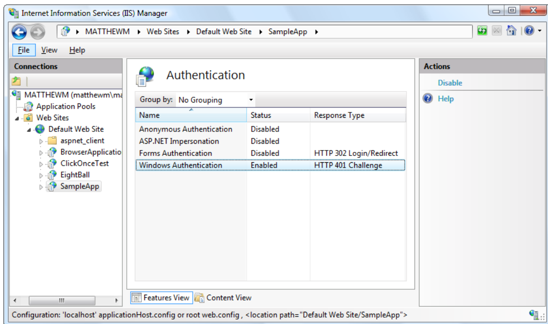
Figure 26-17. Configuring Windows authentication
