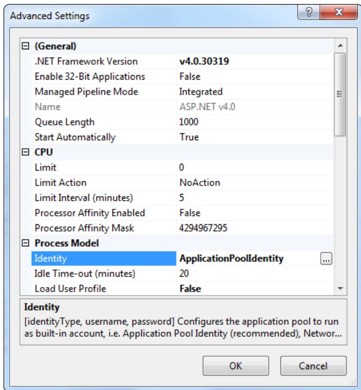
Figure 26-7. Advanced application pool settings
