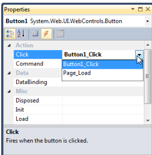
Figure 4-13. Creating or attaching an event handler
