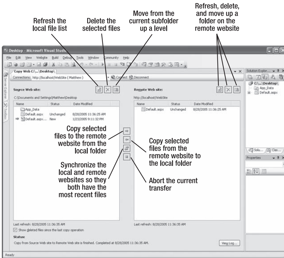
Figure 26-24. Synchronizing a remote website
