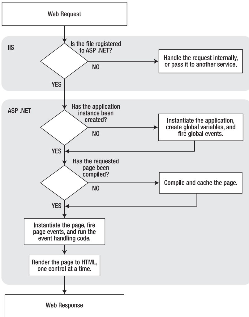
Figure 5-4. The stages in an ASP.NET request
