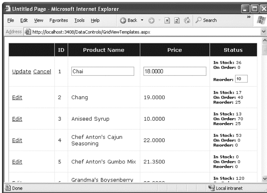
Figure 16-14. Using an edit template
