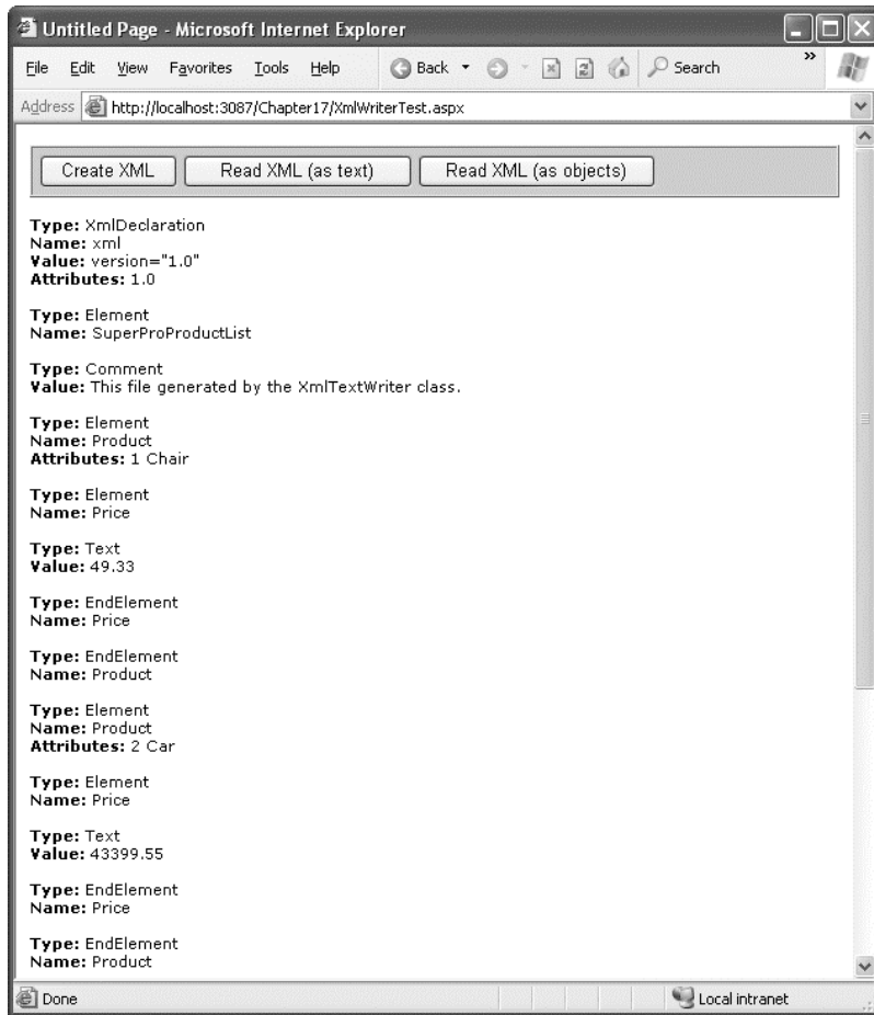
Figure 18-2. Reading XML structure
