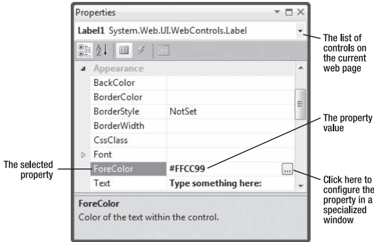
Figure 4-11. The ForeColor property in the Properties window
