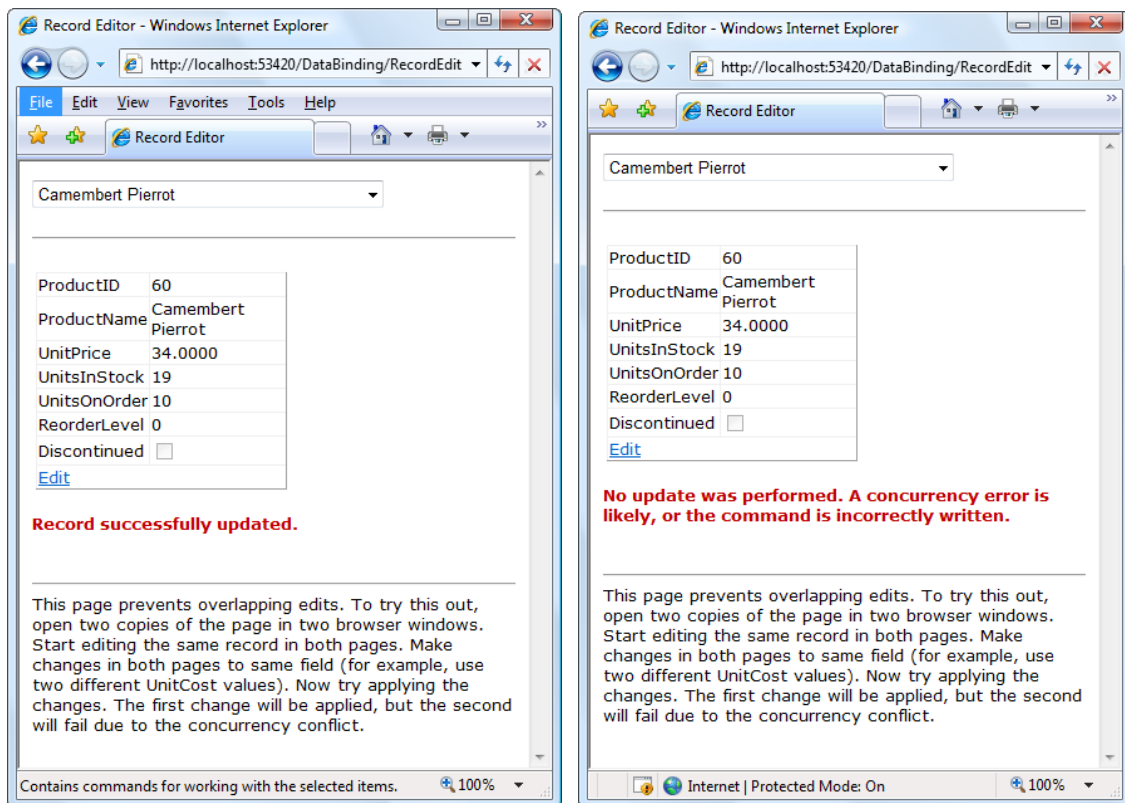
Figure 15-15. A concurrency error in action
