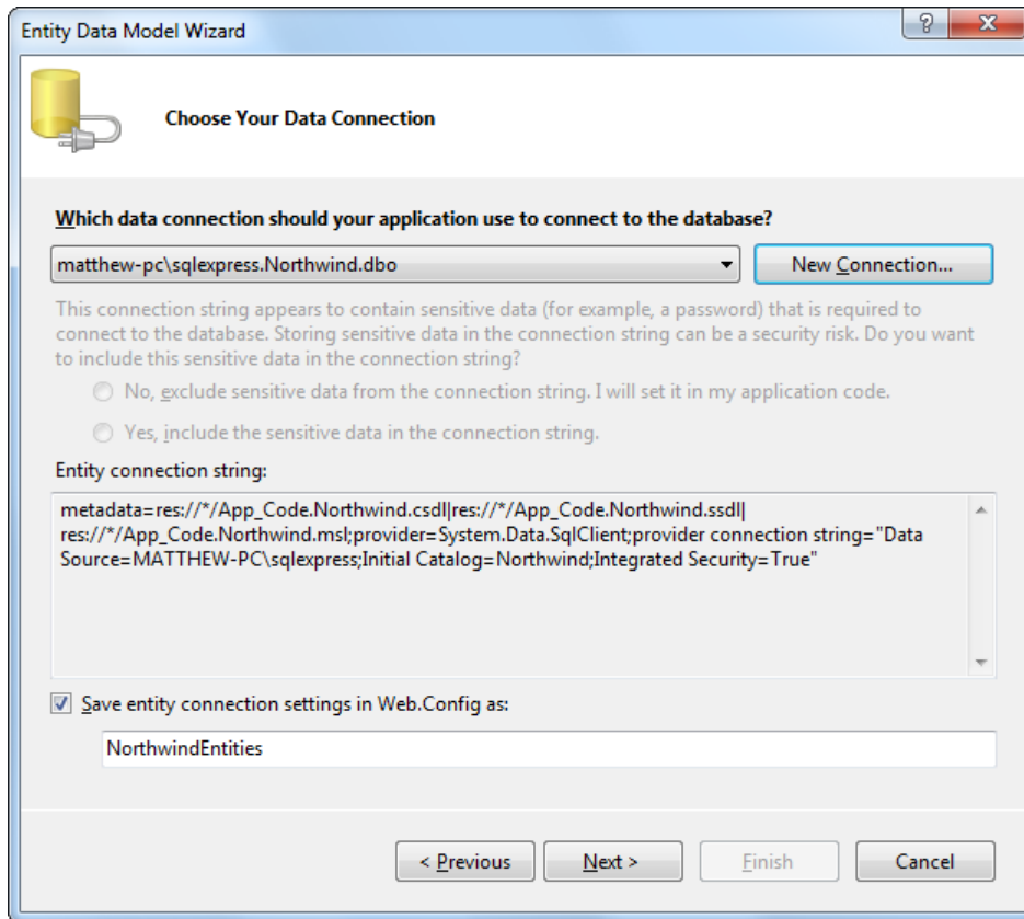
Figure 24-4. Specifying your database connection
