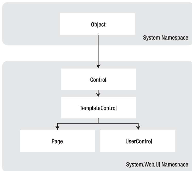
Figure 11-1. The Page and UserControl inheritance chain
