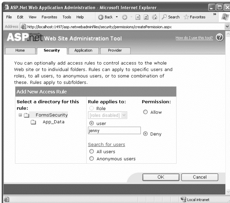
Figure 19-3. Adding an authorization rule
