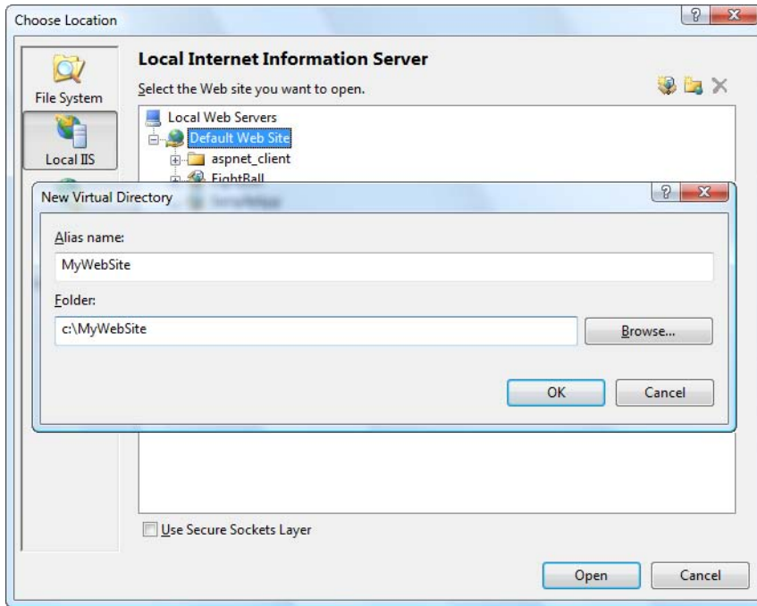
Figure 26-21. Creating a virtual directory in a specific location
