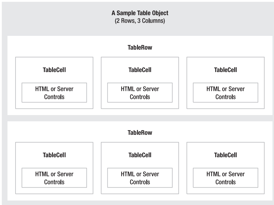
Figure 6-7. Table control containment
