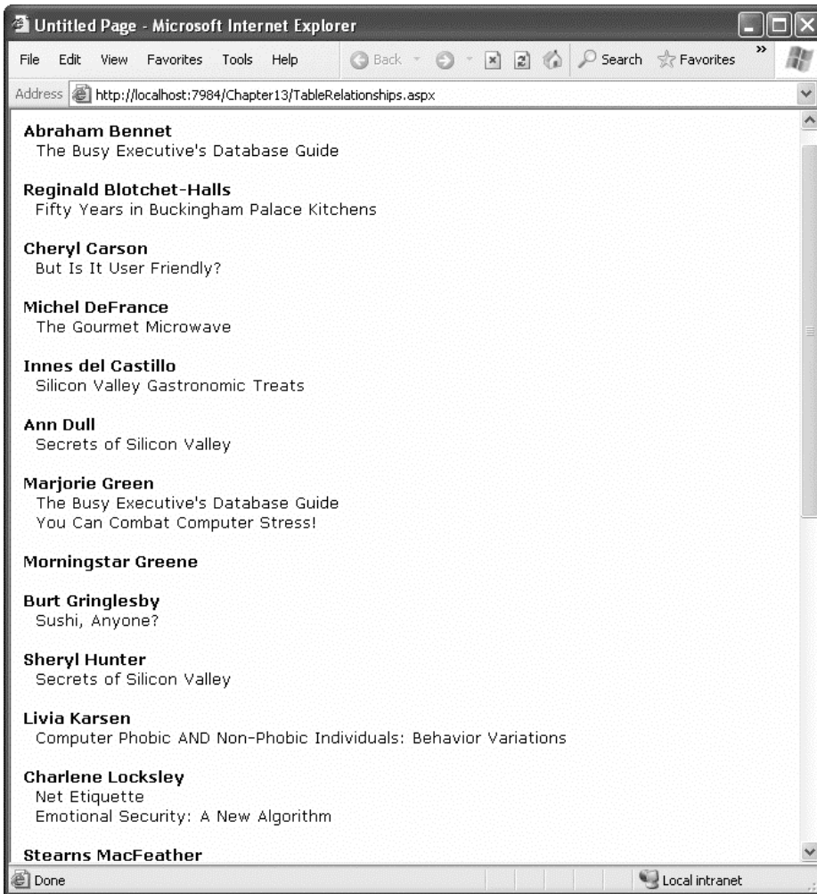
Figure 14-17. Hierarchical information from two tables
