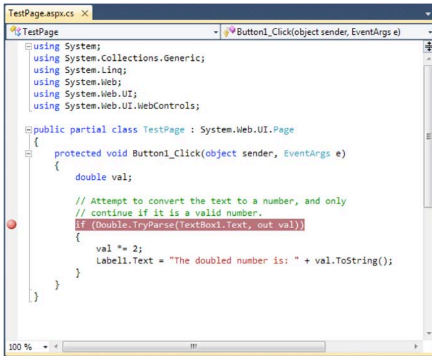
Figure 4-22. Setting a breakpoint
