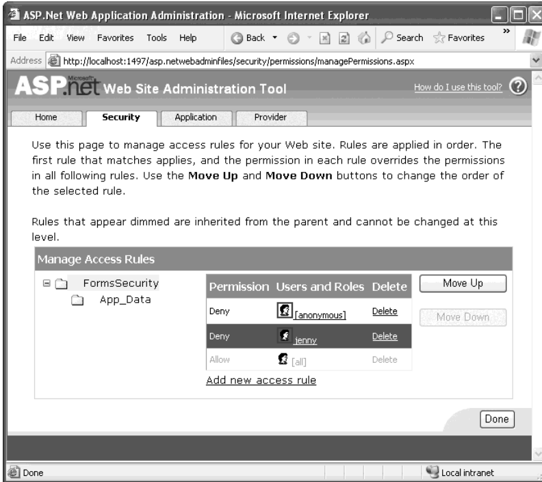
Figure 19-4. Ordering authorization rules
