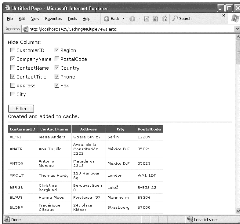
Figure 23-6. Filtering information from a cached DataSet
