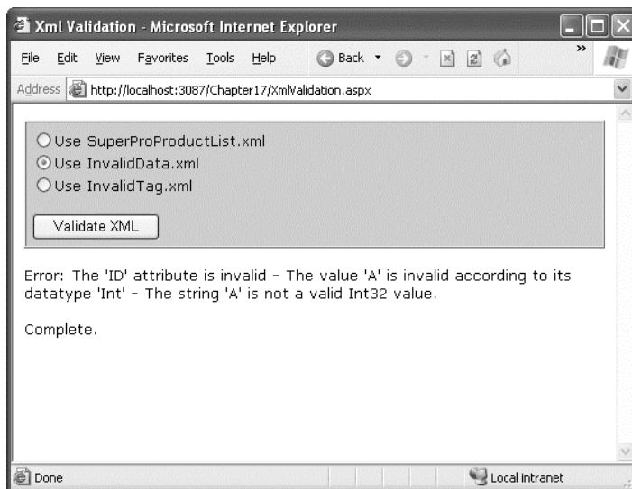
Figure 18-8. The validation test page
