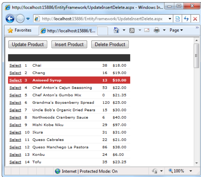
Figure 24-13. Modifying a database with the Entity Framework
