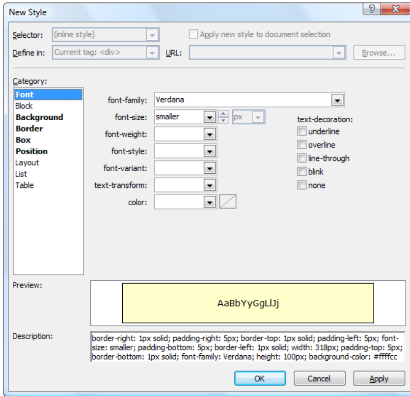
Figure 12-3. Building a styled division
