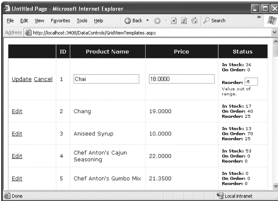
Figure 16-15. Creating an edit template with validation
