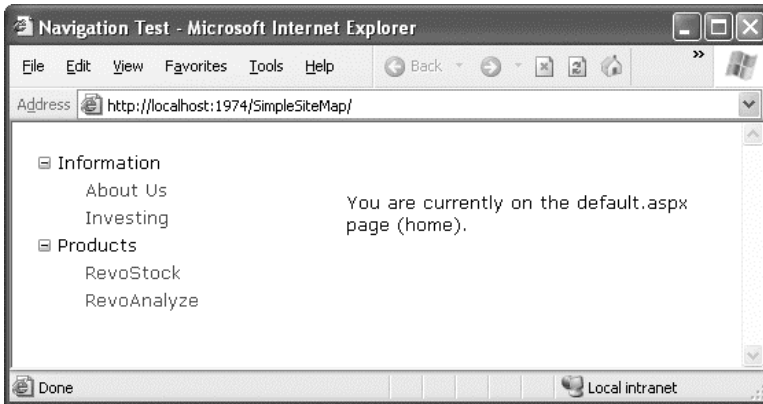
Figure 13-5. A site map without the root node
