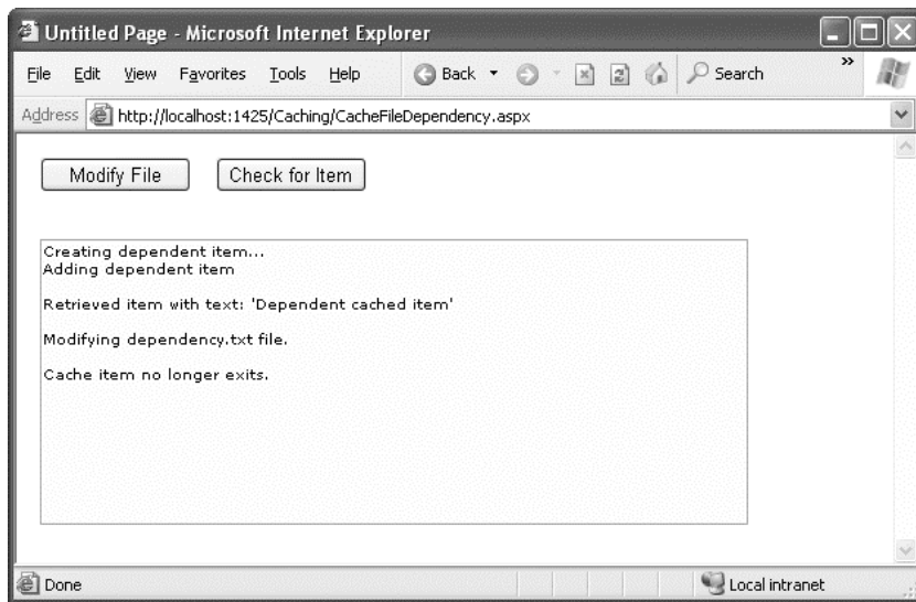
Figure 23-8. Testing cache dependencies
