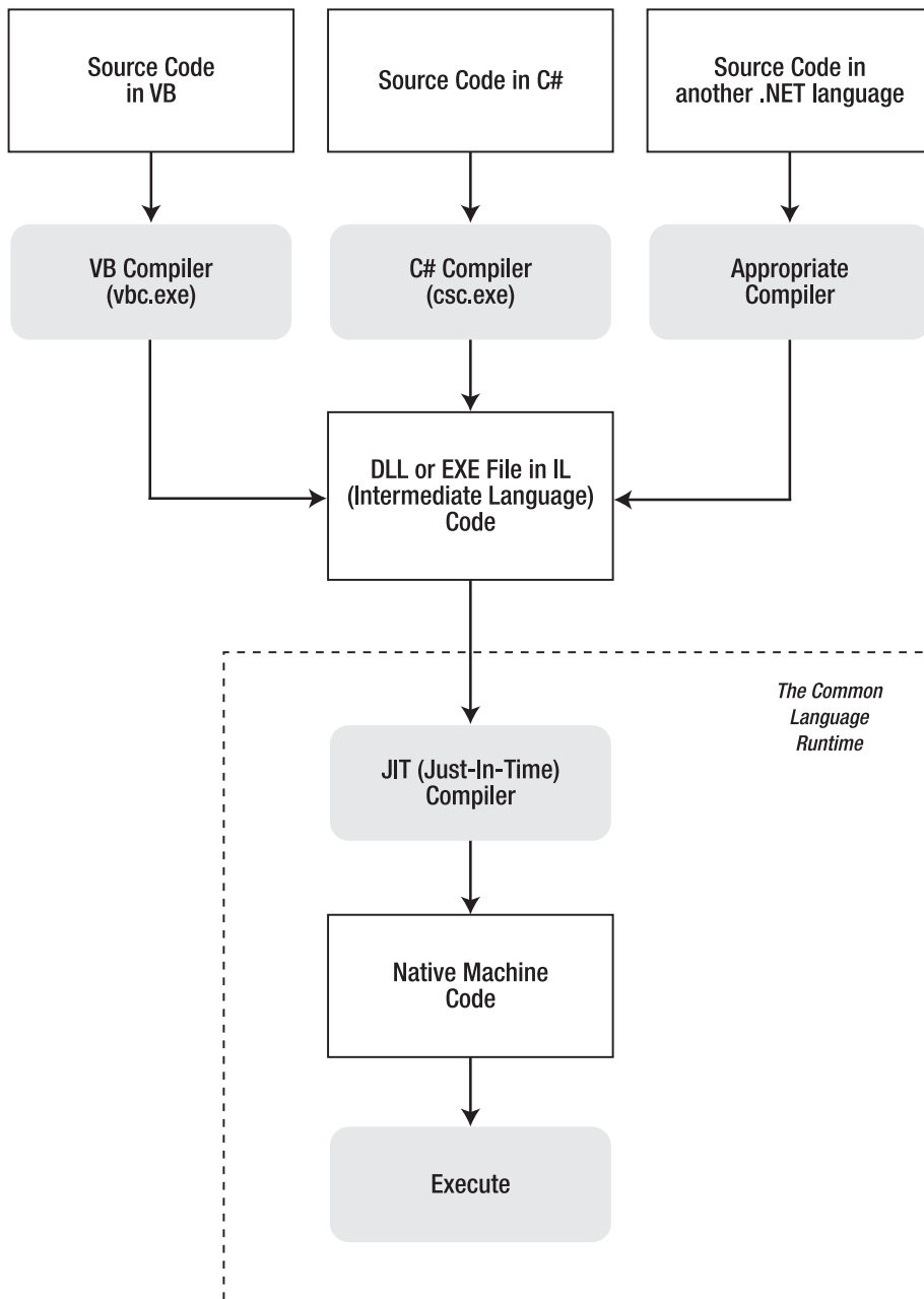
Figure 1-5. Language compilation in .NET
