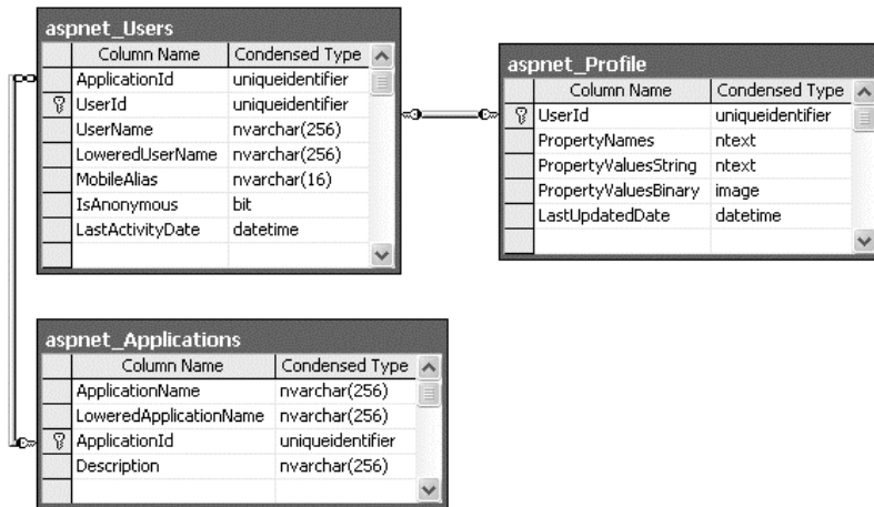
Figure 21-1. The profile tables
