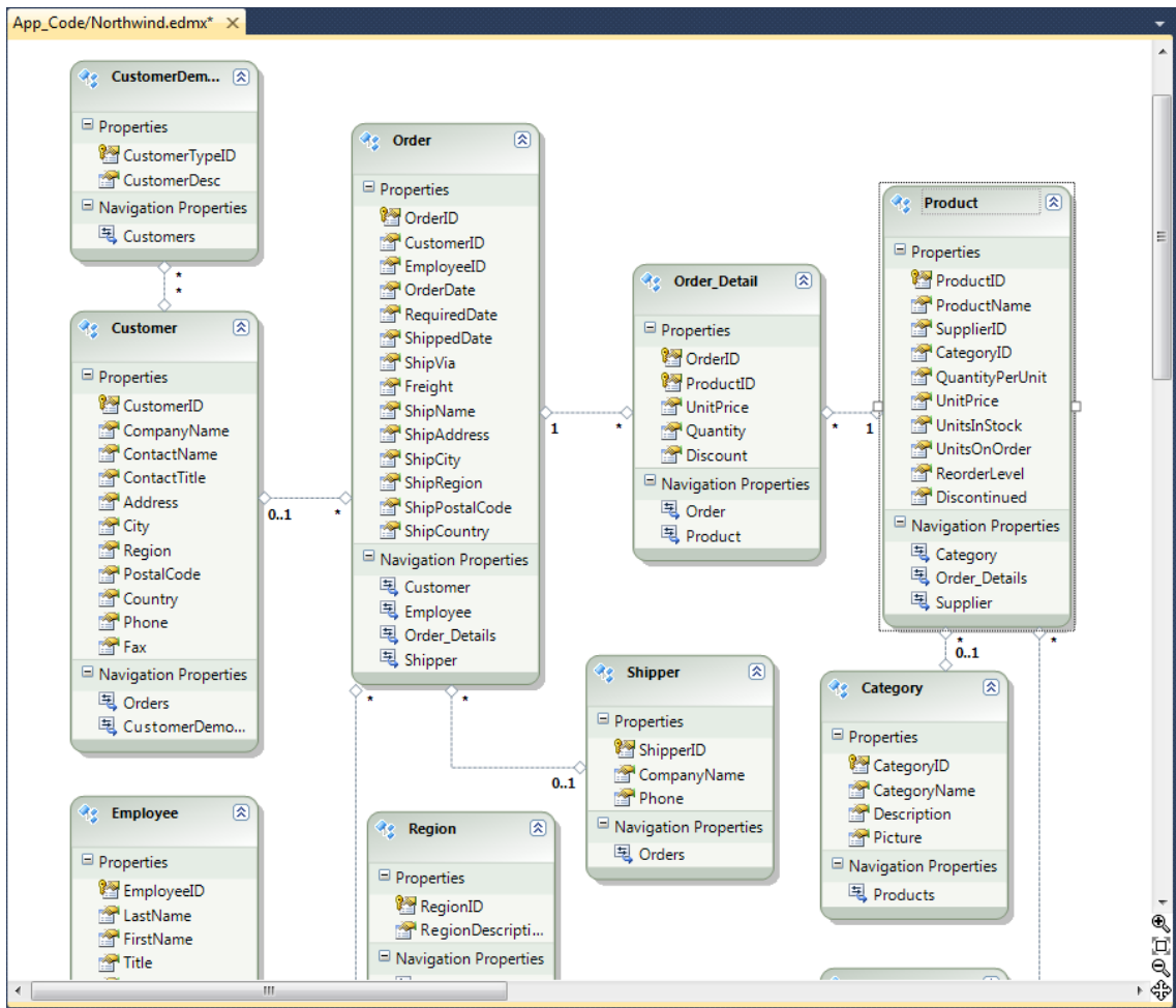
Figure 24-6. Part of the Northwind entity data model
