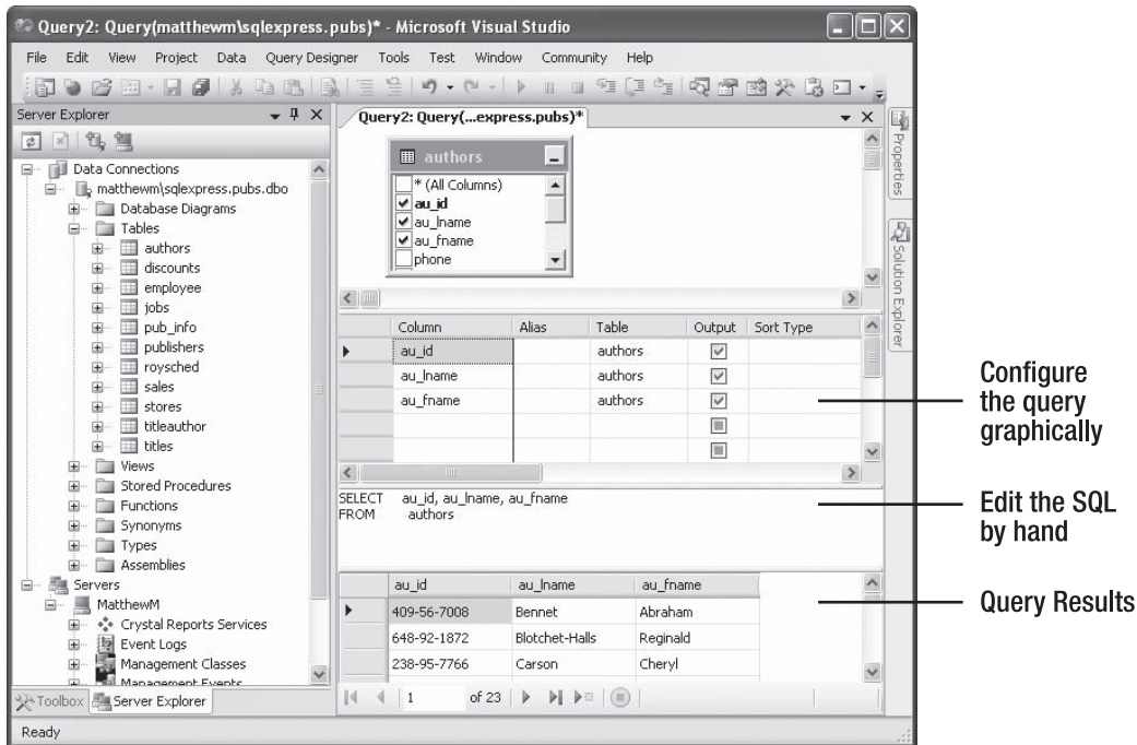
Figure 14-6. Executing a query
