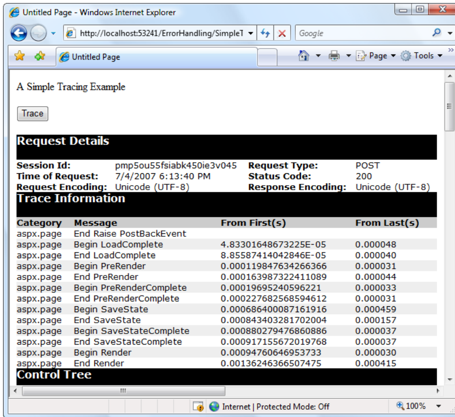
Figure 7-13. Tracing the simple ASP.NET page
