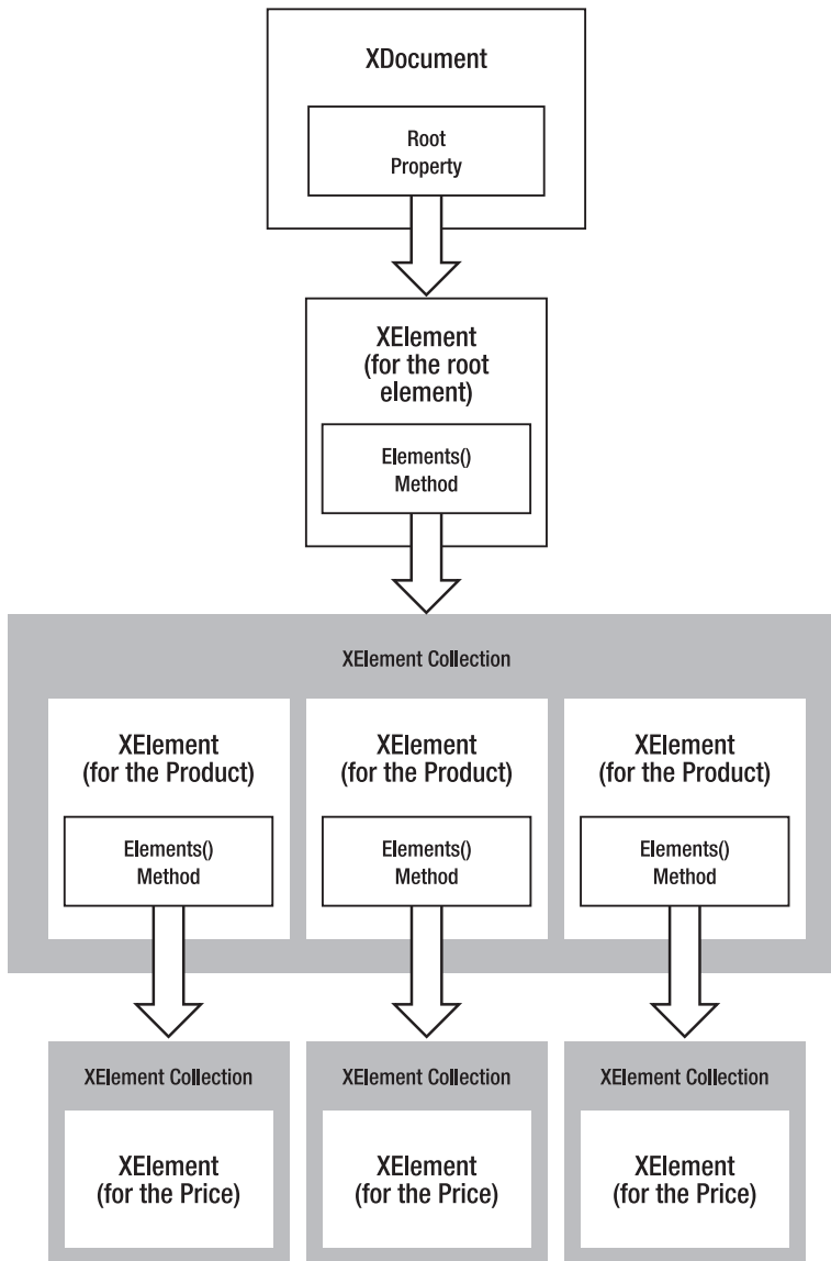
Figure 18-4. An XML document in memory
