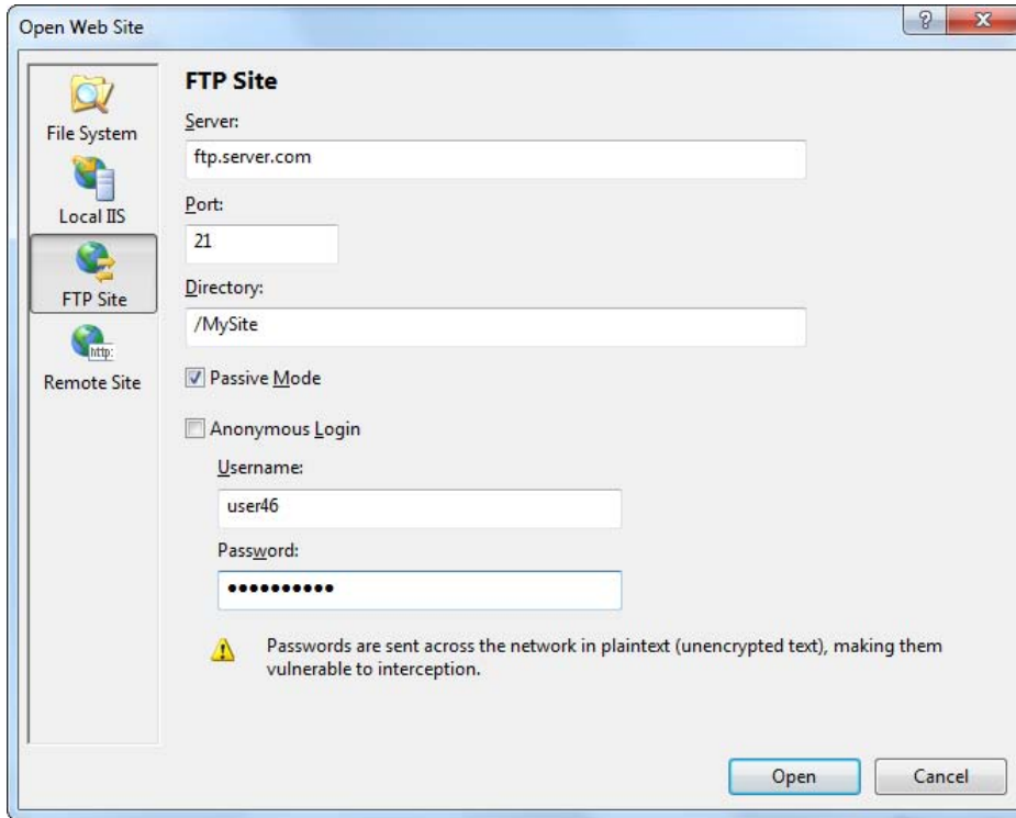
Figure 26-23. Setting the target site
