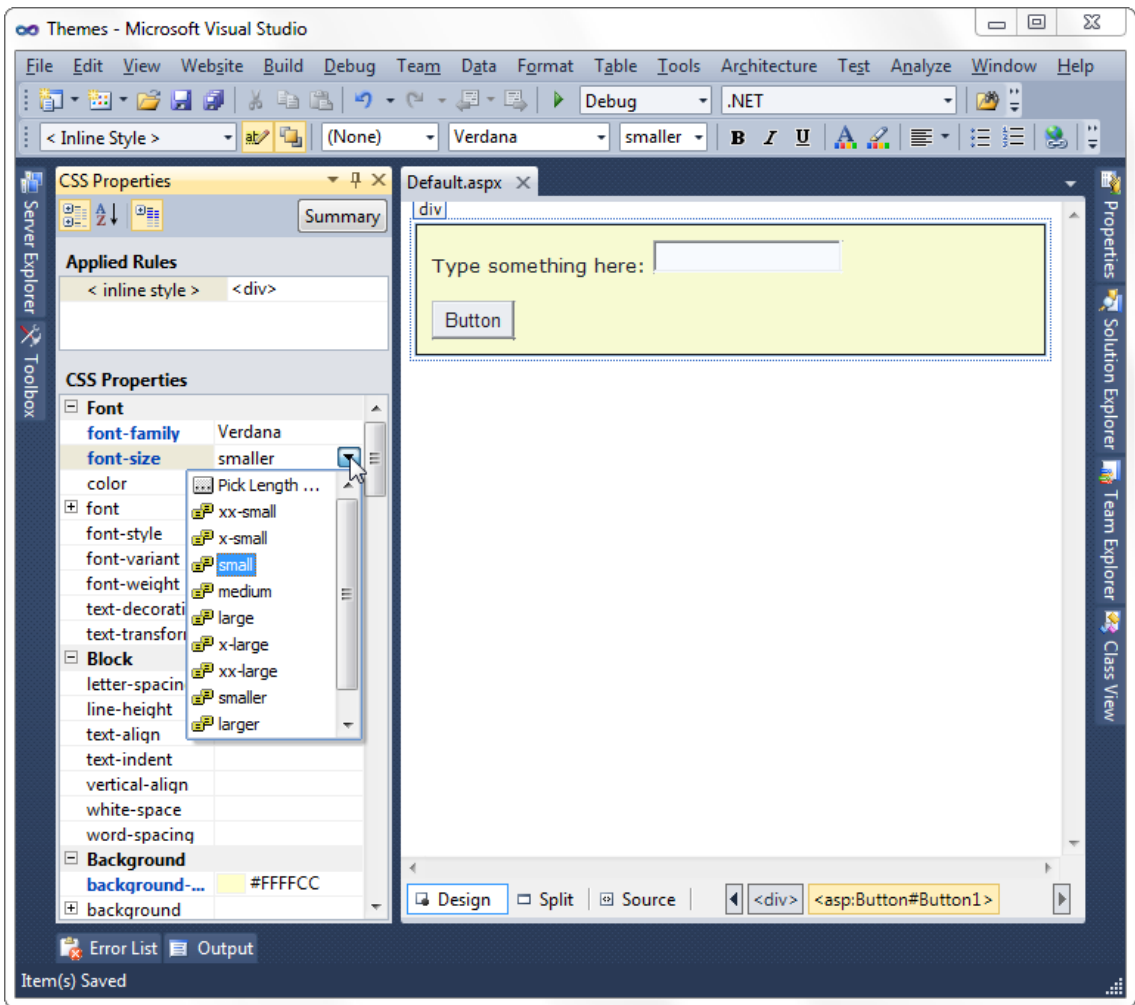
Figure 12-5. The CSS Properties window (on the left)
