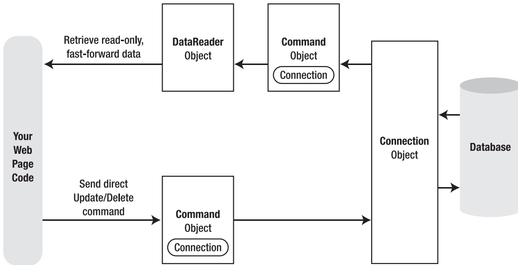
Figure 14-8. Direct data access with ADO.NET
