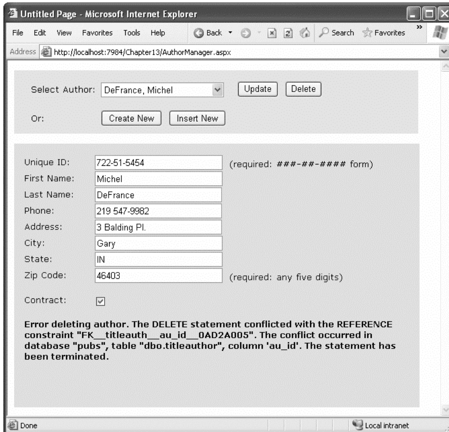
Figure 14-14. A failed delete attempt
