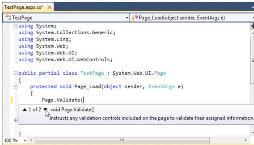
Figure 4-16. IntelliSense with overloaded methods
