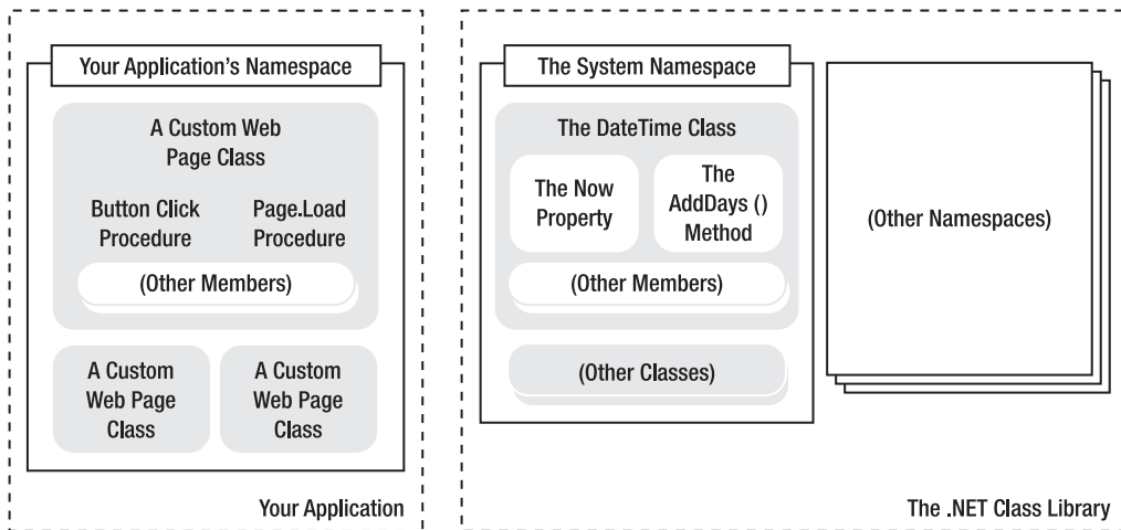
Figure 3-3. A look at two namespaces
