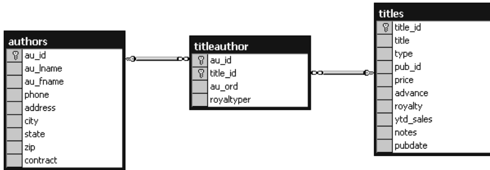
Figure 14-16. A many-to-many relationship
