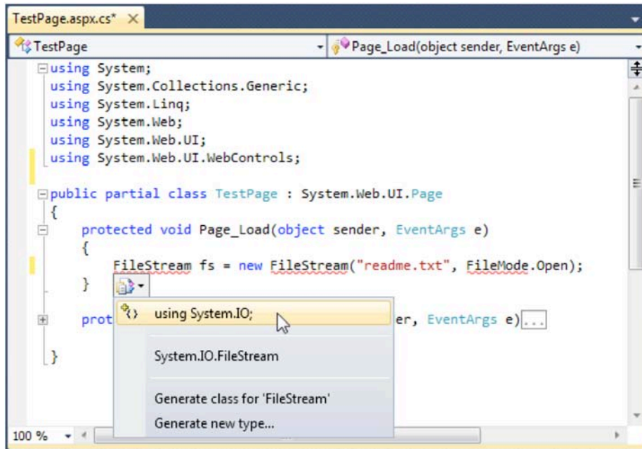
Figure 4-19. Importing a missing namespace
