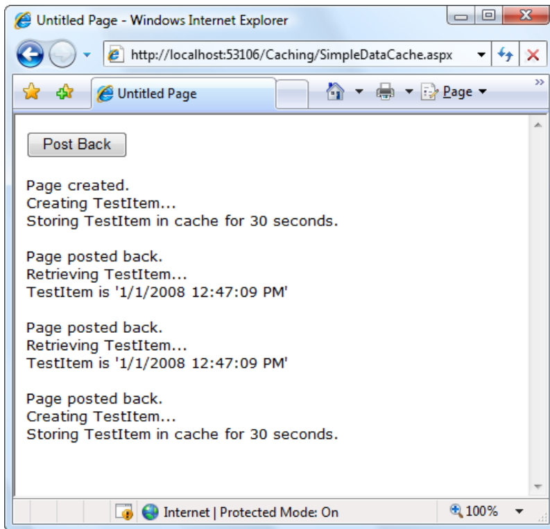
Figure 23-5. A simple cache test
