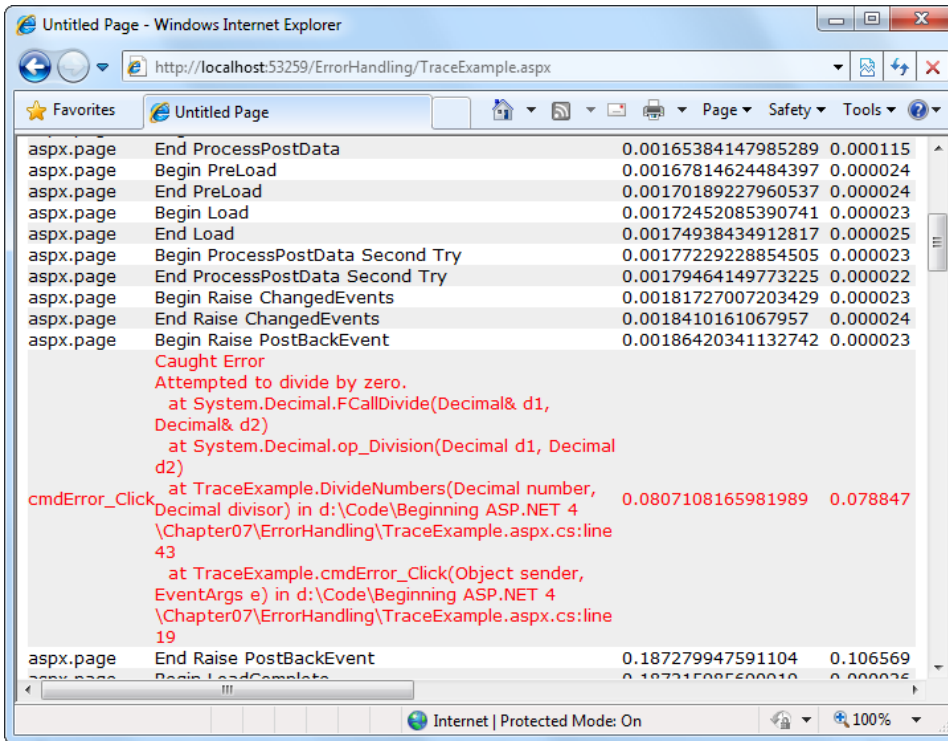
Figure 7-24. An exception trace message
