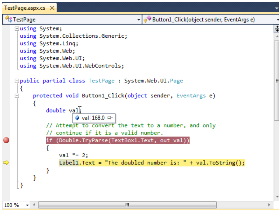
Figure 4-23. Viewing variable contents in break mode
