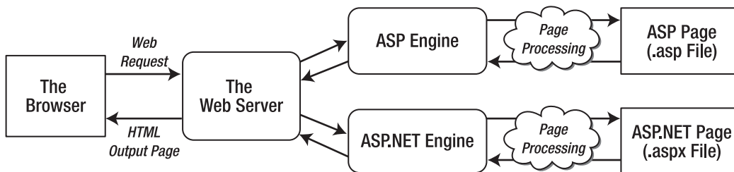
Figure 26-1. How IIS handles a request
