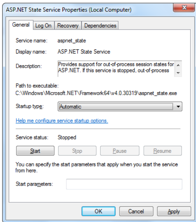
Figure 8-14. Changing the startup type
