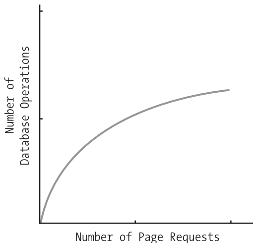
Figure 23-1. The effect of good caching
