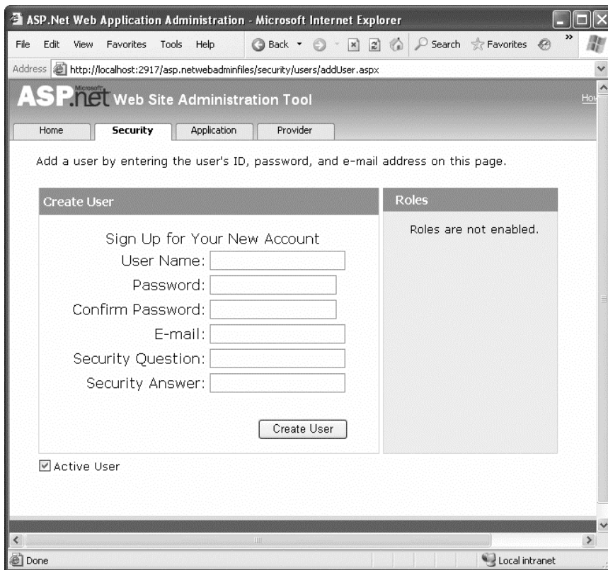
Figure 20-4. Creating a new user
