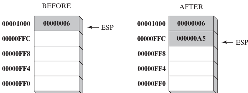
FIGURE 5-5 Pushing Integers on the Stack
