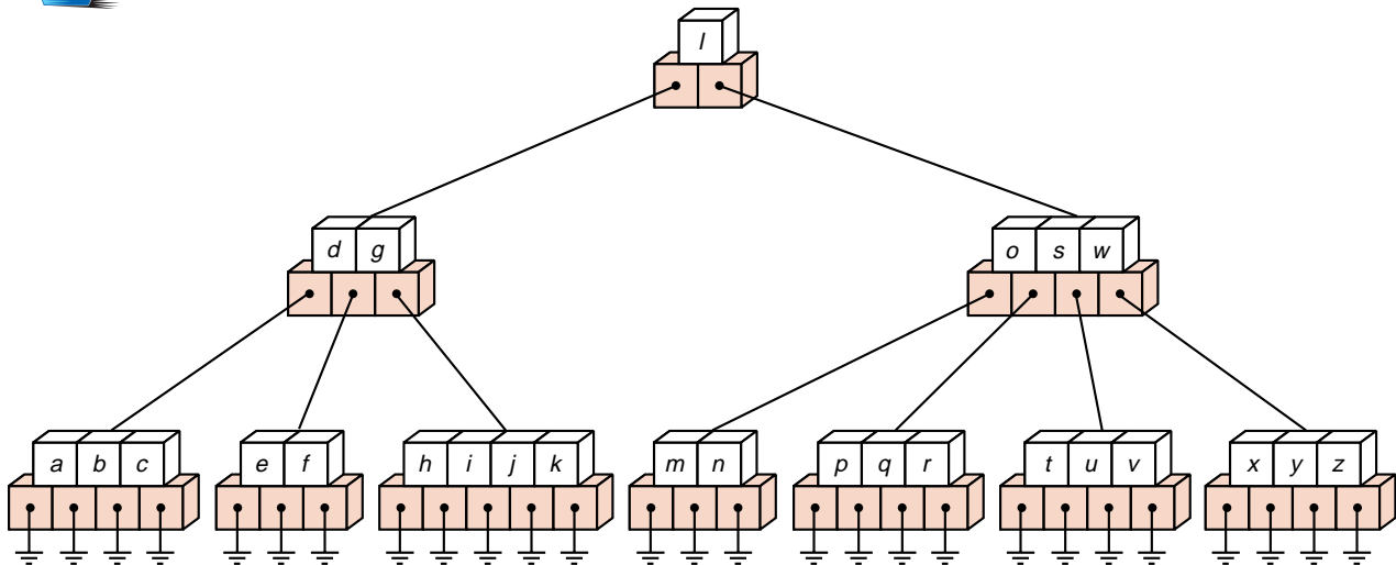
Figure 11.9. A B-tree of order 5
