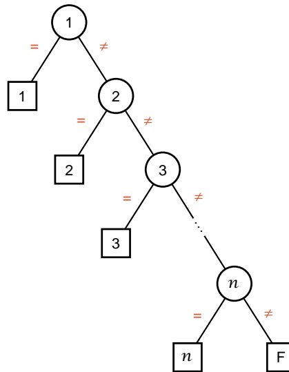
Figure 7.2. Comparison tree for sequential_search
