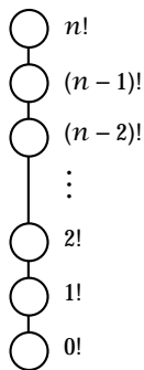
Figure 5.9. Recursion tree for calculating factorials
