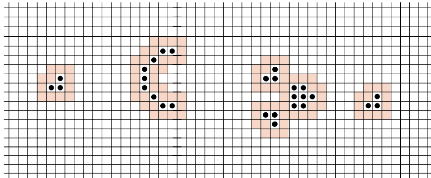
Figure 9.18. A Life configuration with fringe of dead cells
