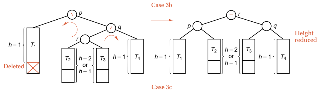
Figure 10.22. Sample cases, removal from an AVL tree
