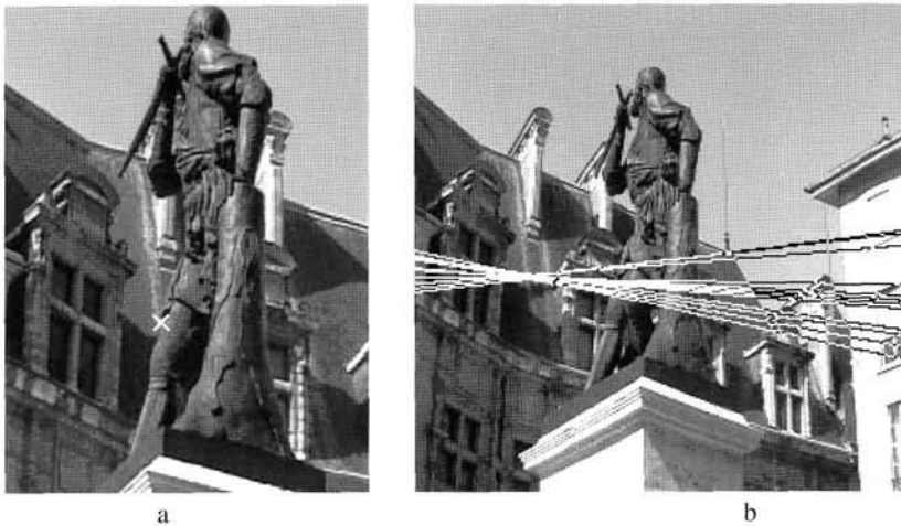
Fig. 11.9. (a) The point in the first image used to compute the epipolar envelopes in the second images. Note the ambiguity of which point is to be found in the second image. The marked point may represent the point on the statue's leg (foreground) or the point on the building behind the statue (background). In the second image, these two points are quite separate, and the epipolar line must pass through them both. (b) Computed corresponding epipolar lines computed from n = 15 point matches. The different lines correspond to different instances of injected noise in the matched points. Gaussian noise of 0.5 pixels in each coordinate was added to the ideal matched point positions before computing the epipolar line corresponding to the selected point. The ML estimator (Gold Standard algorithm) was used to compute F . This experiment shows the basic instability of the computation of the epipolar lines from small numbers of points. To find the point matching the selected point in the image at left, one needs to search over the regions covered by all these epipolar lines.
