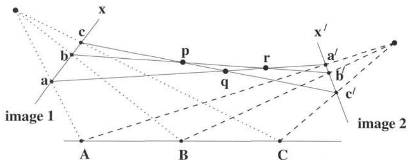
Fig. A7.4. A line projectivity. Points \{a, b, c\} are related to points \{A, B, C\} by a line-to-line perspectivity. Points \{a', b', c'\} are also related to points \{A, B, C\} by a perspectivity. However, points \{a, b, c\} are related to points \{a', b', c'\} by a projectivity; they are not related by a perspectivity because lines joining corresponding points are not concurrent. In fact the pairwise intersections result in three distinct points \{p, q, r\} .
