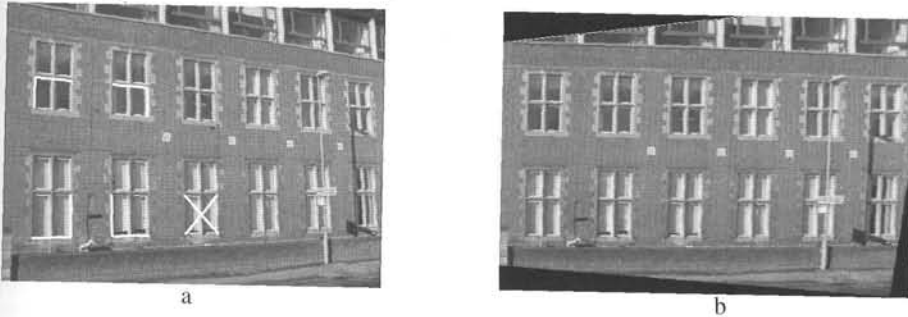
Fig. 2.18. Metric rectification via orthogonal lines II. (a) The conic C_{\infty}^* is determined on the perspective imaged plane (the front wall of the building) using the five orthogonal line pairs shown. The conic C_{\infty}^* determines the circular points, and equivalently the projective transformation necessary to metrically rectify the image (b). The image shown in (a) is the same perspective image as that of figure 2.4(p35), where the perspective distortion was removed by specifying the world position of four image points.
