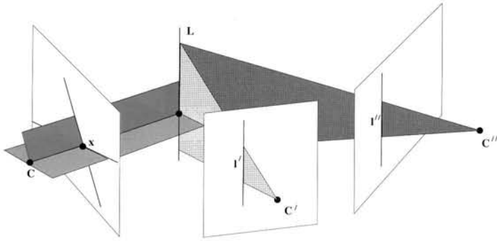
Fig. 17.2. A point–line–line correspondence \mathbf{x} \leftrightarrow l' \leftrightarrow l'' involving three images may be interpreted as follows. Two arbitrary lines are chosen to pass through the point \mathbf{x} in the first image. The four lines then back-project to planes that meet in a point in space.
