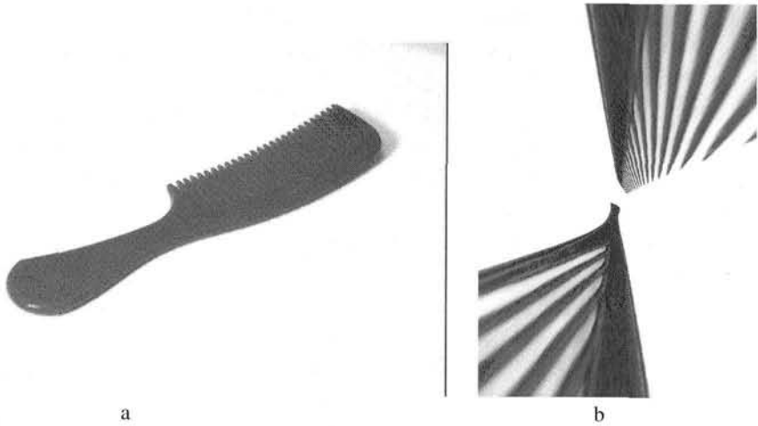
Fig. 21.1. (a) an image of a comb, and (b) the result of applying a projective transformation to the image. The projective transformation does not however preserve the convex hull of the set of points constituting the comb. In the original image, the convex hull of the comb is a finite set contained within the extent of the visible image. However, some of the points in this convex hull are mapped to infinity by the transformation.
