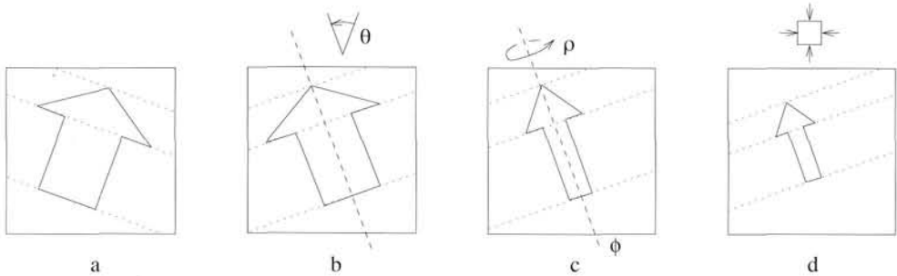
Fig. 14.13. The effect of scale and rotation angles on the epipolar lines for an object moving relative to a stationary camera. This also illustrates the assumed sequence of events accounting for the transition from I_1 to I_2 : (a) I_1 ; (b) cyclotorsion ( \theta ); (c) rotation out of the plane ( \phi and \rho ); (d) scaling, giving I_2 .
