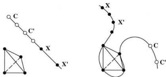
Fig. 22.6. Left: From any centre of projection C, C', \dots lying on the line passing through X and X' , the points X and X' are projected to the same ray. That is, \langle C; \mathbf{E}_i, \mathbf{X} \rangle = \langle C; \mathbf{E}_i, \mathbf{X}' \rangle for all C on the line. Right: The dual statement – all points on the twisted cubic passing through C and C' and the vertices of the reference tetrahedron are projected in the same way relative to the two projection centres. That is, \langle C; \mathbf{E}_i, \mathbf{X} \rangle = \langle C'; \mathbf{E}_i, \mathbf{X} \rangle for all \mathbf{X} on the twisted cubic. This curve is called the horopter for the two centres of projection.
