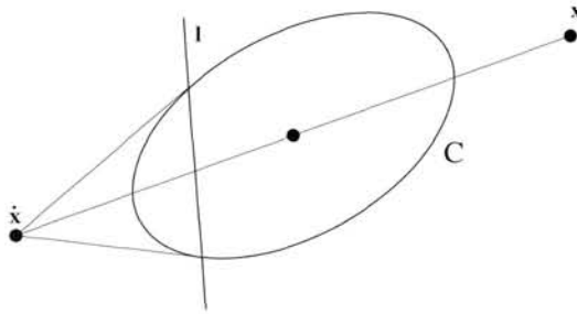
Fig. 8.28. To construct the line perpendicular to the ray through image point x proceed as follows: (i) Reflect x through the centre of C to get point \hat{x} (i.e. at the same distance from the centre as x ). (ii) The desired line is the polar of \hat{x} .
