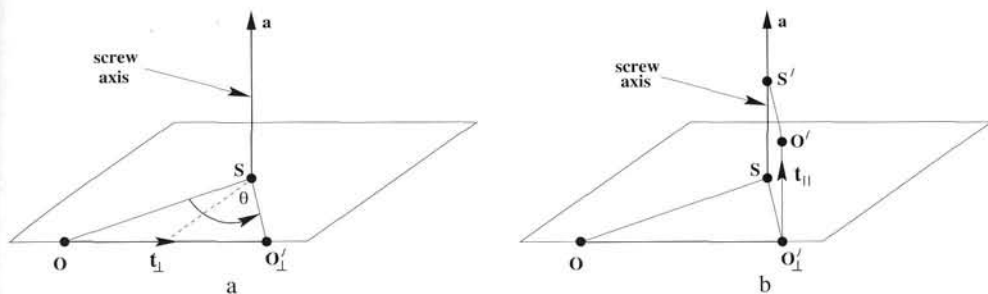
Fig. 3.7. 3D Euclidean motion and the screw decomposition. Any Euclidean rotation R and translation t may be achieved by (a) a rotation about the screw axis, followed by (b) a translation along the screw axis by t_{\parallel} . Here a is the (unit) direction of the rotation axis (so that Ra = a ), and t is decomposed as t = t_{\parallel} + t_{\perp} , which are vector components parallel and orthogonal respectively to the rotation axis direction. The point S is closest to O on the screw axis (so that the line from S to O is perpendicular to the direction of a ). Similarly S' is the point on the screw axis closest to O' .
