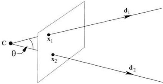
Fig. 8.11. The angle \theta between two rays.
