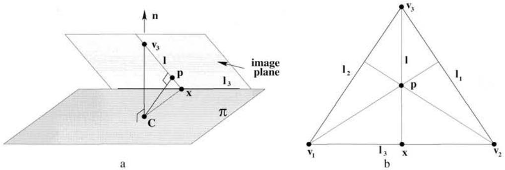
Fig. 8.23. Geometric construction of the principal point. The vanishing line l_3 back-projects to a plane \pi with normal \mathbf{n} . The vanishing point v_3 back-projects to a line orthogonal to the plane \pi . (a) The normal \mathbf{n} of the plane \pi through the camera centre C and the principal axis define a plane, which intersects the image in the line l = \langle v_3, x \rangle . The line l_3 is the intersection of \pi with the image plane, and is also its vanishing line. Clearly the principal point lies on l , and l and l_3 are perpendicular on the image plane. (b) The principal point may be determined from three such constraints as the orthocentre of the triangle.
