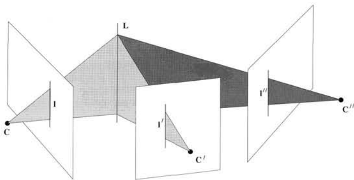
Fig. 15.1. A line L in 3-space is imaged as the corresponding triplet I \leftrightarrow I' \leftrightarrow I'' in three views indicated by their centres, C, C', C'' , and image planes. Conversely, corresponding lines back-projected from the first, second and third images all intersect in a single 3D line in space.
