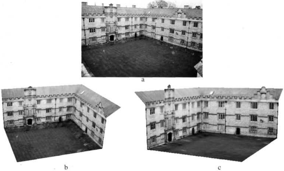
Fig. 8.26. Single view reconstruction. (a) Original image of the Fellows quad, Merton College, Oxford. (b) (c) Views of the 3D model created from the single image. The vanishing line of the roof planes is computed from the repetition of the texture pattern.
