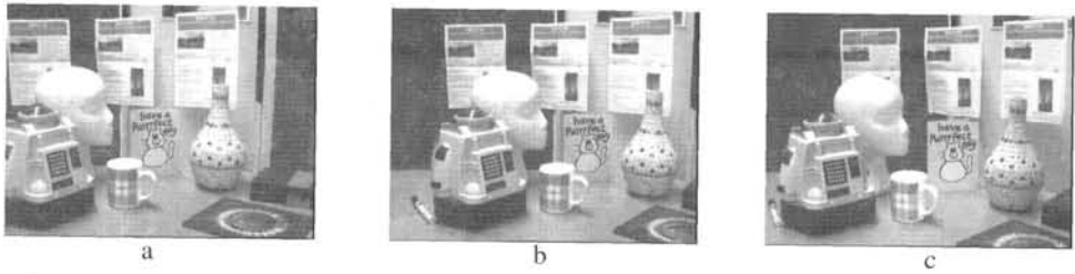
Fig. 8.6. Between images (a) and (b) the camera rotates about the camera centre. Corresponding points (that is images of the same 3D point) are related by a plane projective transformation. Note that 3D points at different depths which are coincident in image (a), such as the mug lip and cat body, are also coincident in (b), so there is no motion parallax in this case. However, between images (a) and (c) the camera rotates about the camera centre and translates. Under this general motion coincident points of differing depth in (a) are imaged at different points in (c), so there is motion parallax in this case due to the camera translation.
