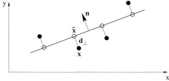
Fig. 14.4. In 2D a line is the analogue of the hyperplane defined by F_A , and the problem of estimating the true correspondence given a measured correspondence, is the problem of determining the closest point (\hat{x}, \hat{y}) on the line ax + by + c to a measurement point (x, y) . The normal to the line has direction (a, b) , and the perpendicular distance of the point (x, y) from the line is d_{\perp} = (ax + by + c)/\sqrt{a^2 + b^2} , so that (\hat{x}, \hat{y})^T = (x, y)^T - d_{\perp} \hat{n} , where \hat{n} = (a, b)/\sqrt{a^2 + b^2} .
