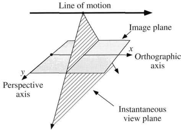
Fig. 6.9. Acquisition geometry of a pushbroom camera.
