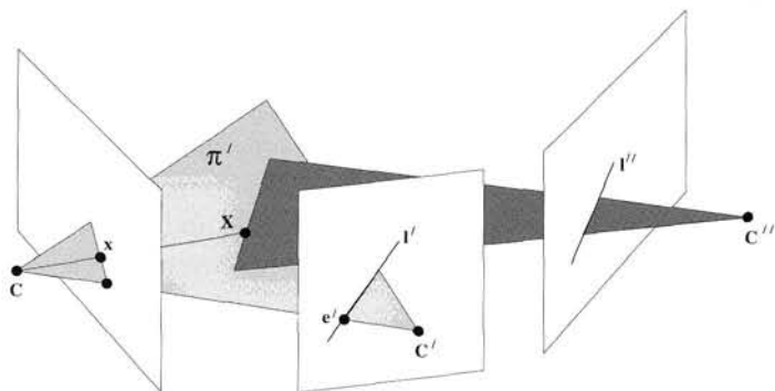
Fig. 15.6. If the plane \pi' defined by l' is an epipolar plane for the first two views, then any line l'' in the third view gives a point-line-line incidence.
