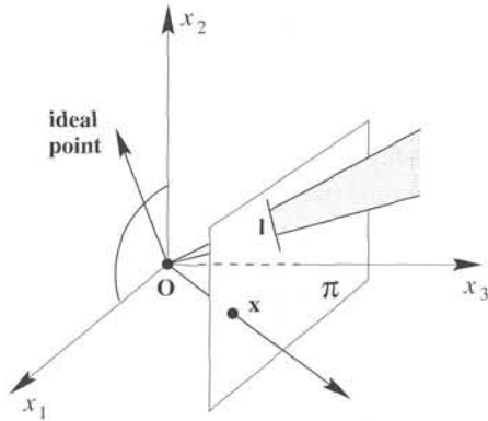
Fig. 2.1. A model of the projective plane. Points and lines of \mathbb{IP}^2 are represented by rays and planes, respectively, through the origin in \mathbb{R}^3 . Lines lying in the x_1x_2 -plane represent ideal points, and the x_1x_2 -plane represents l_\infty .
