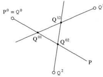
Fig. 22.7. Configuration of the three camera centres and the three ambiguous points. If the three points Q^{ij} are distinct, then they all lie in the plane of the camera centres C_{Q^i}^j .
