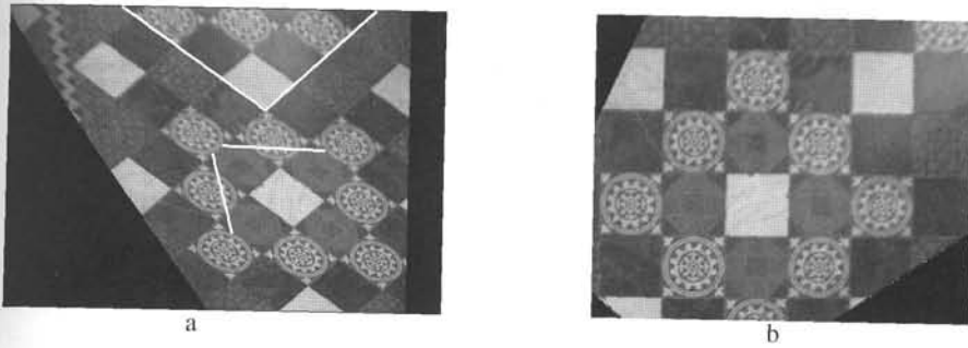
Fig. 2.17. Metric rectification via orthogonal lines I. The affine transformation required to metrically rectify an affine image may be computed from imaged orthogonal lines. (a) Two (non-parallel) line pairs identified on the affinely rectified image (figure 2.13) correspond to orthogonal lines on the world plane. (b) The metrically rectified image. Note that in the metrically rectified image all lines orthogonal in the world are orthogonal, world squares have unit aspect ratio, and world circles are circular.
