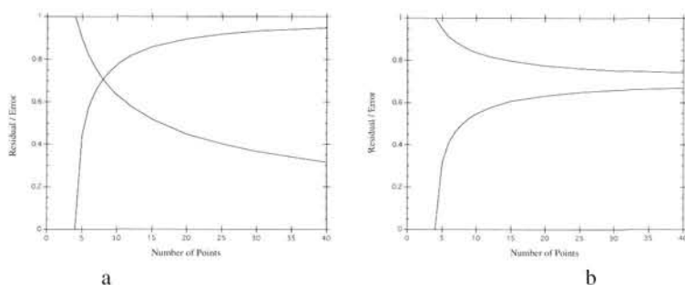
Fig. 5.3. Optimal error when noise is present in (a) one image, and in (b) both images as the number of points varies. An error level of one pixel is assumed. The descending curve shows the estimation error \epsilon_{\text{est}} and the ascending curve shows the residual error \epsilon_{\text{res}} .
