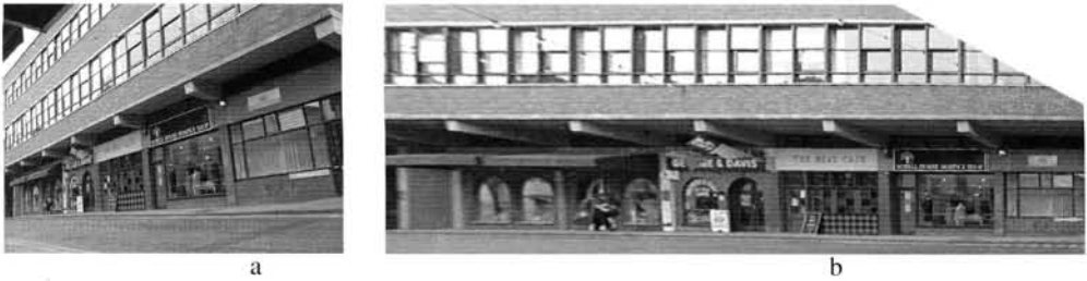
Fig. 8.25. Plane rectification via partial internal parameters (a) Original image. (b) Rectification assuming the camera has square pixels and principal point at the centre of the image. The focal length is computed from the single orthogonal vanishing point pair. The aspect ratio of a window in the rectified image differs from the ground truth value by 3.7%. Note that the two parallel planes, the upper building facade and the lower shopfront, are both mapped to fronto-parallel planes.
