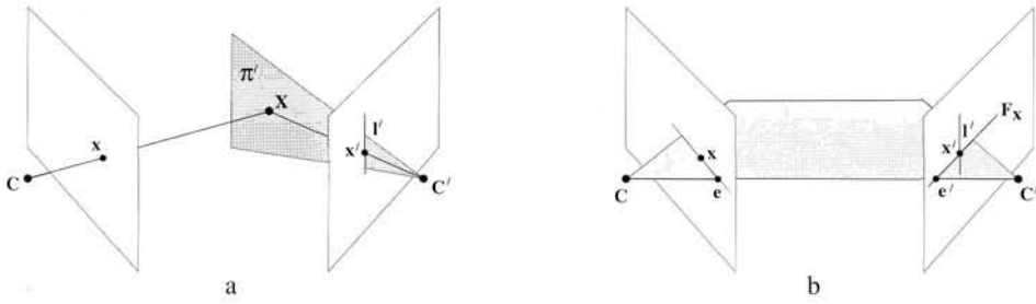
Fig. 13.6. A degenerate homography. (a) The map induced by a plane through the second camera centre is a degenerate homography H = [Y']_x F . The plane \pi' intersects the second image plane in the line Y' . All points in the first view are mapped to points on Y' in the second. (b) A point x in the first view is imaged at x' , the intersection of Y' with the epipolar line Fx of x , so that x' = Y' \times Fx .
