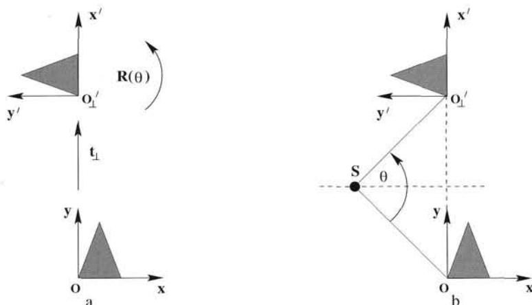
Fig. 3.6. 2D Euclidean motion and a "screw" axis. (a) The frame \{x, y\} undergoes a translation t_{\perp} and a rotation by \theta to reach the frame \{x', y'\} . The motion is in the plane orthogonal to the rotation axis. (b) This motion is equivalent to a single rotation about the screw axis S . The screw axis lies on the perpendicular bisector of the line joining corresponding points, such that the angle between the lines joining S to the corresponding points is \theta . In the figure the corresponding points are the two frame origins and \theta has the value 90^{\circ} .
