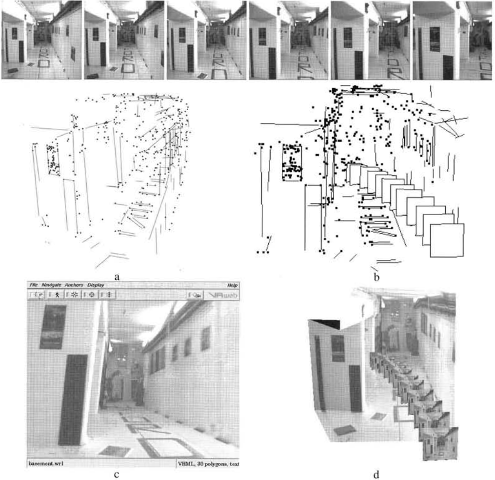
Fig. 18.3. Corridor sequence. (a) A three dimensional reconstruction of points and lines in the scene, and (b) cameras (represented by their image planes) computed automatically from the images. A texture mapped triangulated graphical model is then automatically constructed as described in [Baillard-99]. (c) A rendering of the scene from a novel viewpoint, different from any in the sequence. (d) VRML model of the scene with the cameras represented by their image planes (texture mapped with the original images from the sequence).
