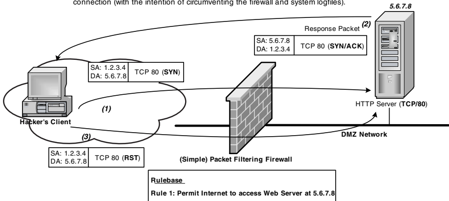
Exhibit 15. TCP Ping Scan
