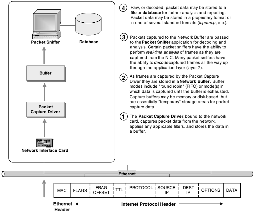
Exhibit 15. IP Packet Sniffer Operation
