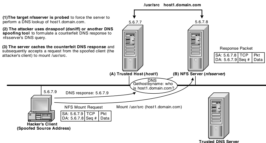
Exhibit 14. NFS (IP) Spoofing
