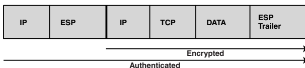
Exhibit 38. IPSec VPN Packet
