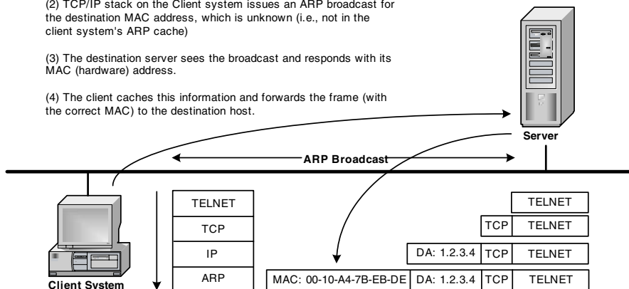
Exhibit 2. ARP Resolution
