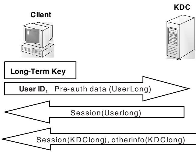
Exhibit 13. Initial Authentication
