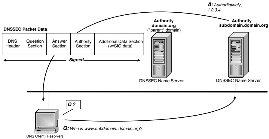
Exhibit 22. DNSSEC Operation
