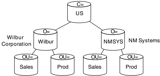
Exhibit 1. X.500 Tree
