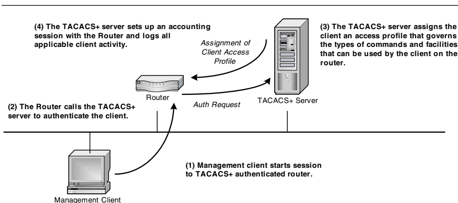
Exhibit 28. TACACS+ Authentication
