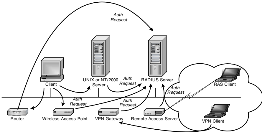
Exhibit 27. RADIUS Authentication
