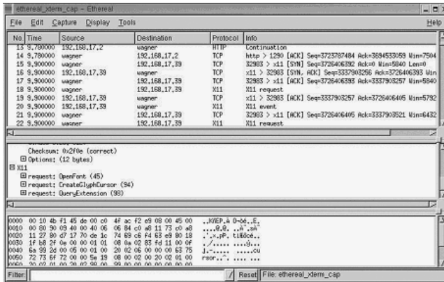
Exhibit 14. Packet Capture
