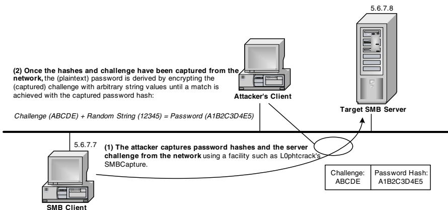
Exhibit 3. SMBCapture
