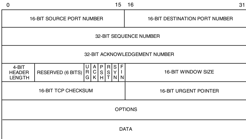
Exhibit 18. TCP Segment
