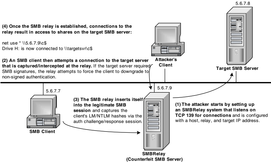
Exhibit 16. SMBRelay
