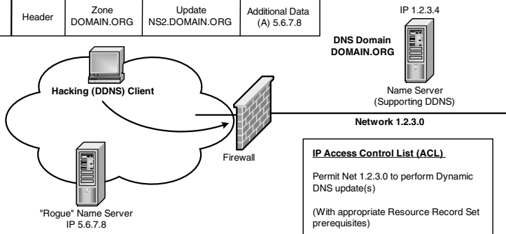
Exhibit 12. DDNS Spoofing
