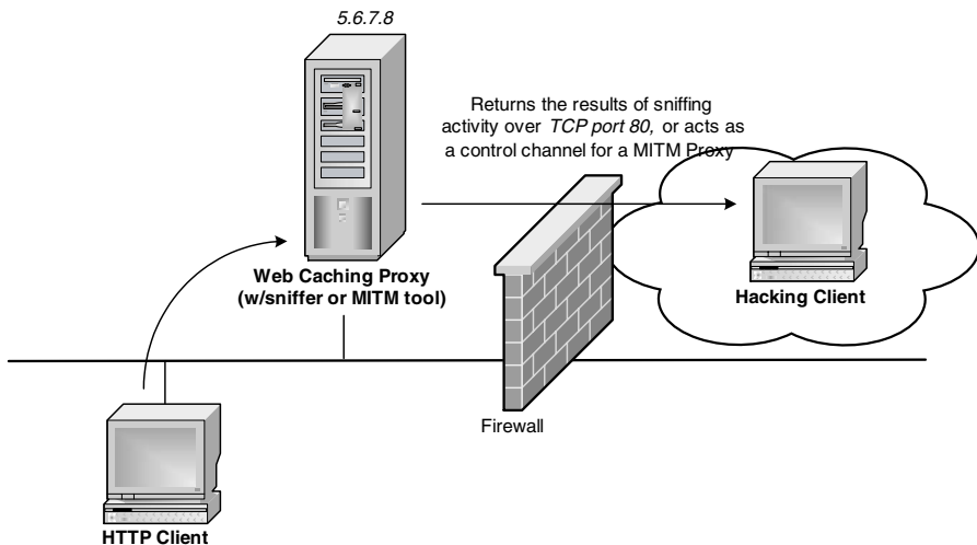
Exhibit 12. Man-in-the-Middle Attack
