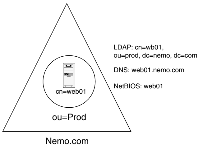
Exhibit 12. Naming Standards
