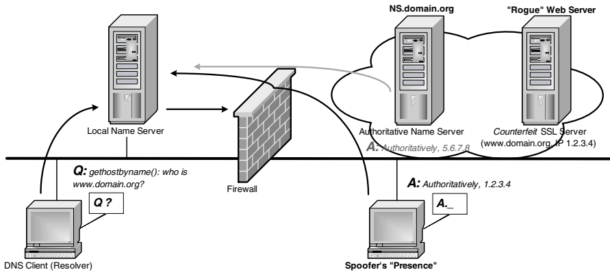
Exhibit 17. HTTP Redirection
