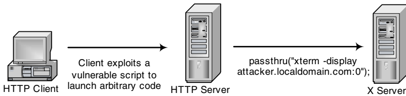
Exhibit 42. X-Term Exploit
