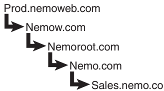
Exhibit 11. Domain Trees
