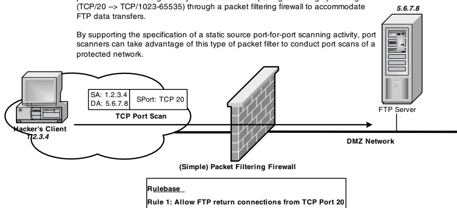
Exhibit 22. Source Port Scanning
