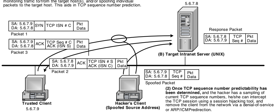
Exhibit 25. IP Session Hijacking/TCP Sequence Number Prediction
