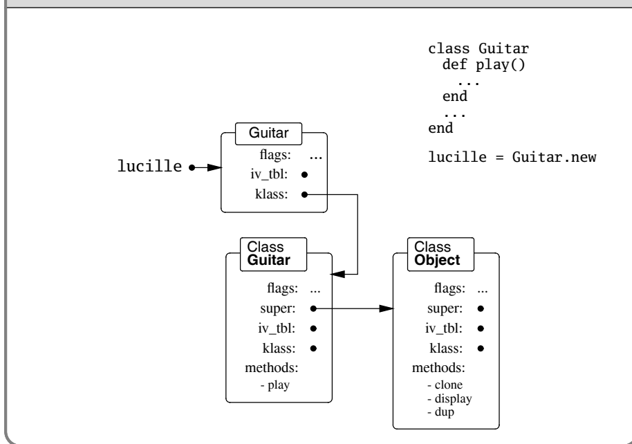
Figure 24.1. A basic object, with its class and superclass
