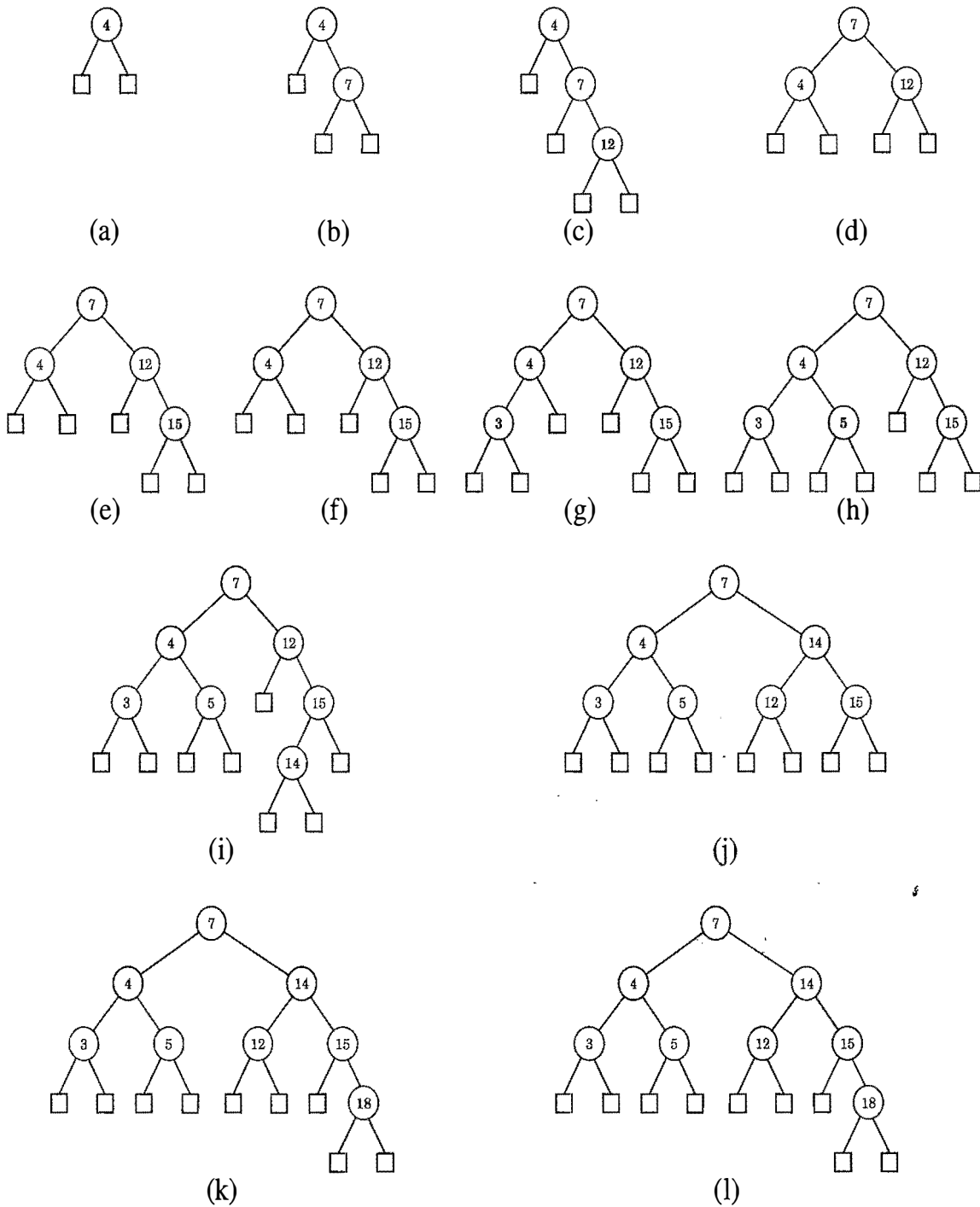
Figure 10.30: A sequence of insertions in a red-black tree: (a) initial tree; (b) insertion of 7; (c) insertion of 12, which causes a double red; (d) after restructuring; (e) insertion of 15, which causes a double red; (f) after recoloring (the root remains black); (g) insertion of 3; (h) insertion of 5; (i) insertion of 14, which causes a double red; (j) after restructuring; (k) insertion of 18, which causes a double red; (l) after recoloring. (Continues in Figure 10.31.)
