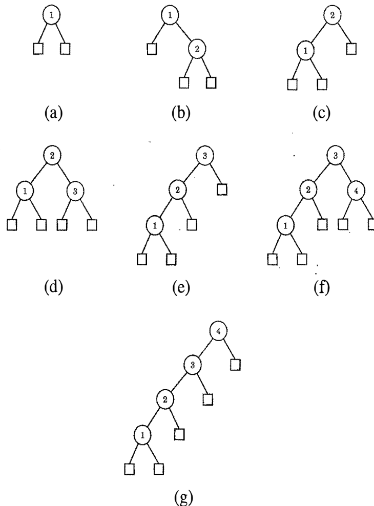
Figure 10.17: A sequence of insertions in a splay tree: (a) initial tree; (b) after inserting 2; (c) after splaying; (d) after inserting 3; (e) after splaying; (f) after inserting 4; (g) after splaying.
