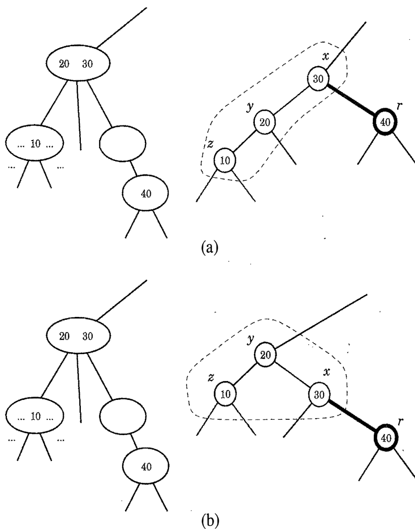
Figure 10.35: Adjustment of a red-black tree in the presence of a double black problem: (a) configuration before the adjustment and corresponding nodes in the associated (2,4) tree (a symmetric configuration is possible); (b) configuration after the adjustment with the same corresponding nodes in the associated (2,4) tree.
