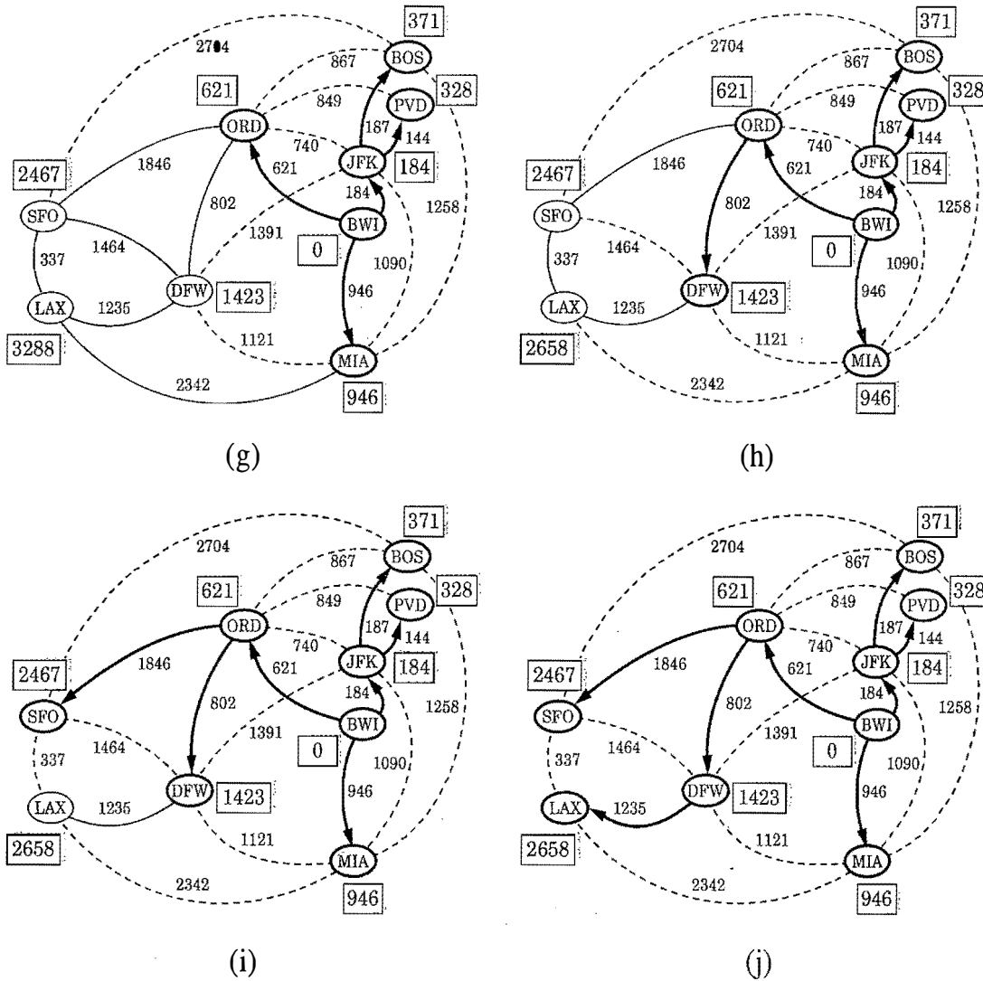
Figure 13.15: An example execution of Dijkstra’s algorithm. (Continued from Figure 13.14.)
