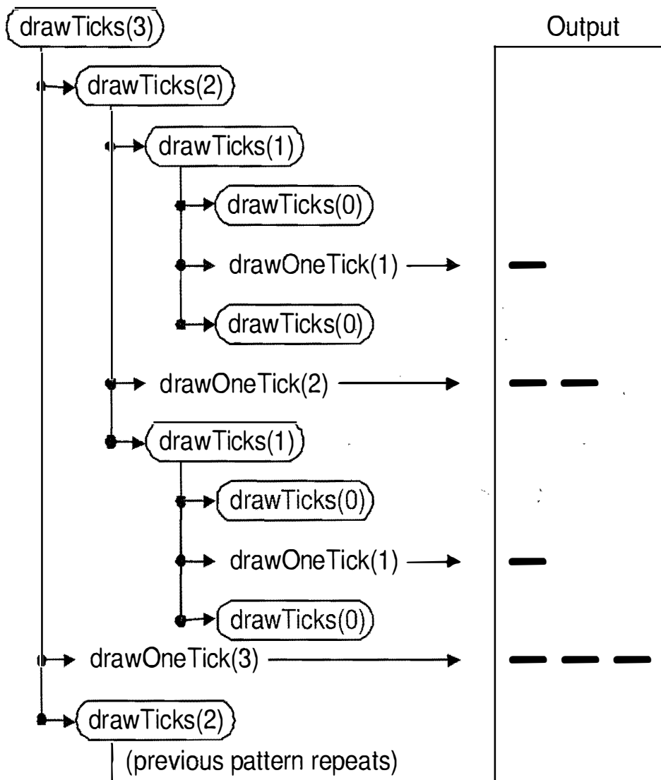
Figure 3.23: A partial recursion trace for the call drawTicks(3) . The second pattern of calls for drawTicks(2) is not shown, but it is identical to the first.
