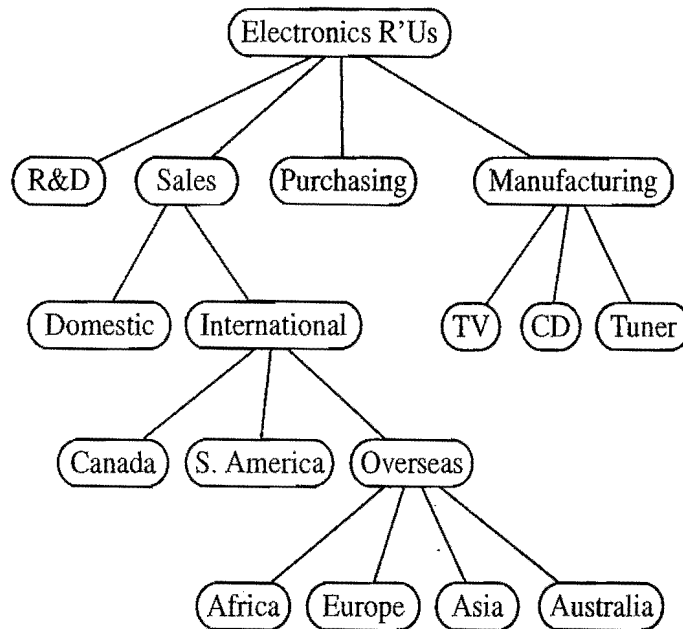
Figure 7.2: A tree with 17 nodes representing the organization of a fictitious corporation. The root stores Electronics R'Us . The children of the root store R&D , Sales , Purchasing , and Manufacturing . The internal nodes store Sales , International , Overseas , Electronics R'Us , and Manufacturing .
