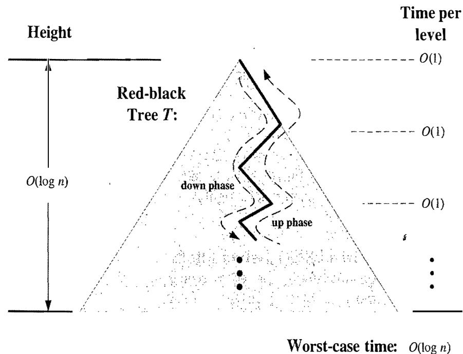
Figure 10.38: Illustrating the running time of searches and updates in a red-black tree. The time performance is O(1) per level, broken into a down phase, which typically involves searching, and an up phase, which typically involves recolorings and performing local trinode restructurings (rotations).
