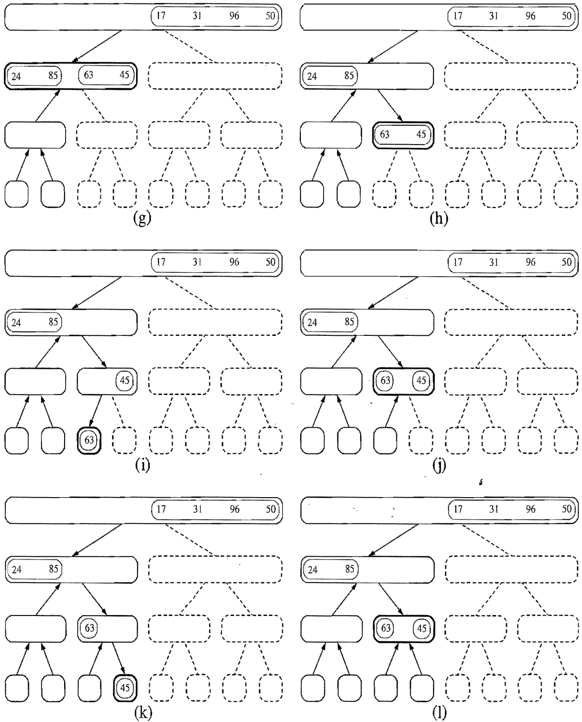
Figure 11.3: Visualization of an execution of merge-sort. (Continues in Figure 11.4.)
