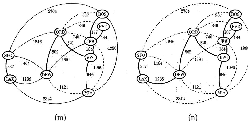
Figure 13.20: Example of an execution of Kruskal's MST algorithm (continued). The edge considered in (n) merges the last two clusters, which concludes this execution of Kruskal's algorithm. (Continued from Figure 13.19.)
