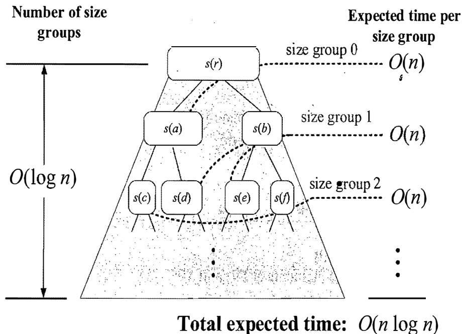
Figure 11.13: A visual time analysis of the quick-sort tree T . Each node is shown labeled with the size of its subproblem.
