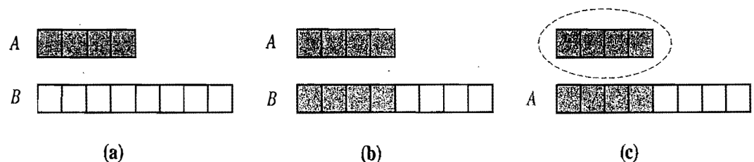
Figure 6.2: An illustration of the three steps for “growing” an extendable array: (a) create new array B ; (b) copy elements from A to B ; (c) reassign reference A to the new array. Not shown is the future garbage collection of the old array.
