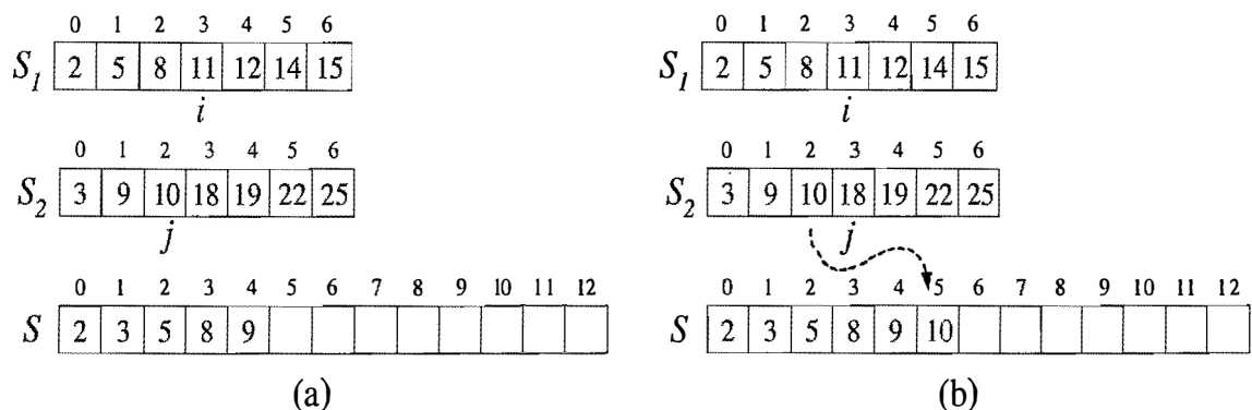
Figure 11.5: A step in the merge of two sorted arrays. We show the arrays before the copy step in (a) and after it in (b).
