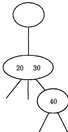
Figure 10.34: Recoloring of a red-black tree that propagates the double black problem: (a) configuration before the recoloring and corresponding nodes in the associated (2,4) tree before the fusion (other similar configurations are possible); (b) configuration after the recoloring and corresponding nodes in the associated (2,4) tree after the fusion.
