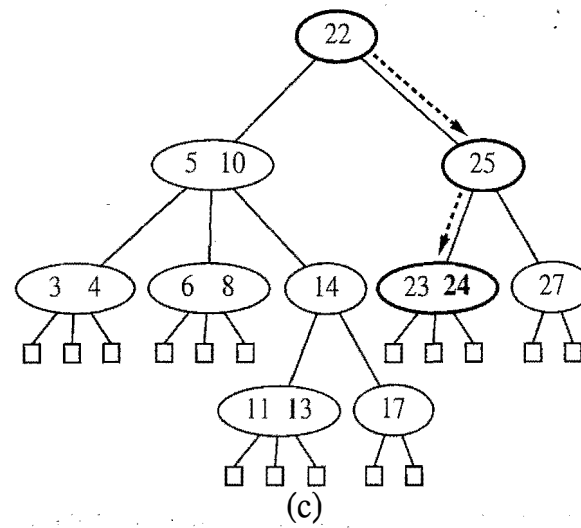
Figure 10.19: (a) A multi-way search tree T ; (b) search path in T for key 12 (unsuccessful search); (c) search path in T for key 24 (successful search).
