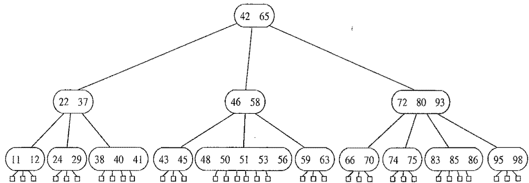
Figure 14.6: A B-tree of order 6.
