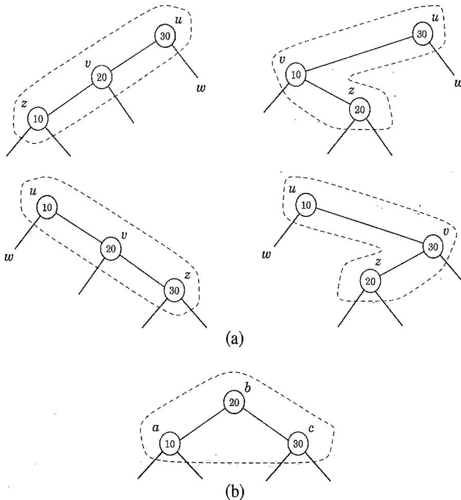
Figure 10.28: Restructuring a red-black tree to remedy a double red: (a) the four configurations for u , v , and z before restructuring; (b) after restructuring.
