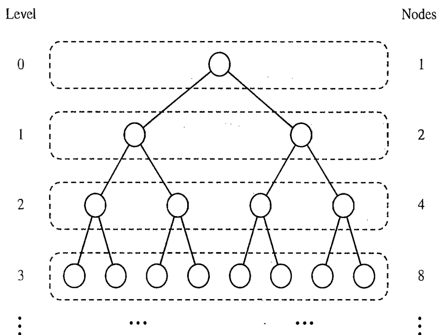
Figure 7.12: Maximum number of nodes in the levels of a binary tree.
