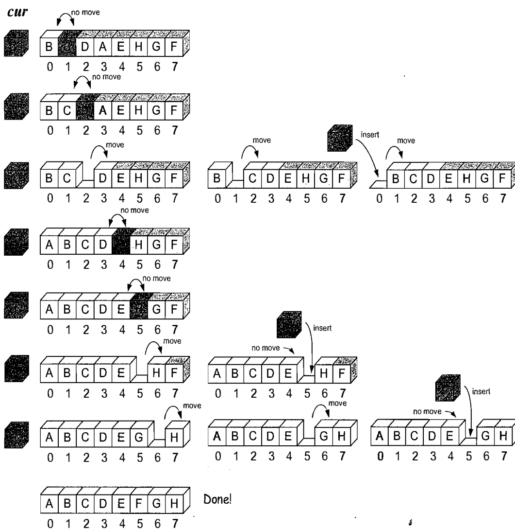
Figure 3.5: Execution of the insertion-sort algorithm on an array of eight characters. We show the completed (sorted) part of the array in white, and we color the next element that is being inserted into the sorted part of the array with light blue. We also highlight that character on the left, since it is stored in the cur variable. Each row corresponds to an iteration of the outer loop, and each copy of the array in a row corresponds to an iteration of the inner loop. Each comparison is shown with an arc. In addition, we indicate whether that comparison resulted in a move or not.
