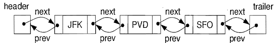
Figure 3.14: A doubly linked list with sentinels, header and trailer, marking the ends of the list. An empty list would have these sentinels pointing to each other. We do not show the null prev pointer for the header nor do we show the null next pointer for the trailer.
