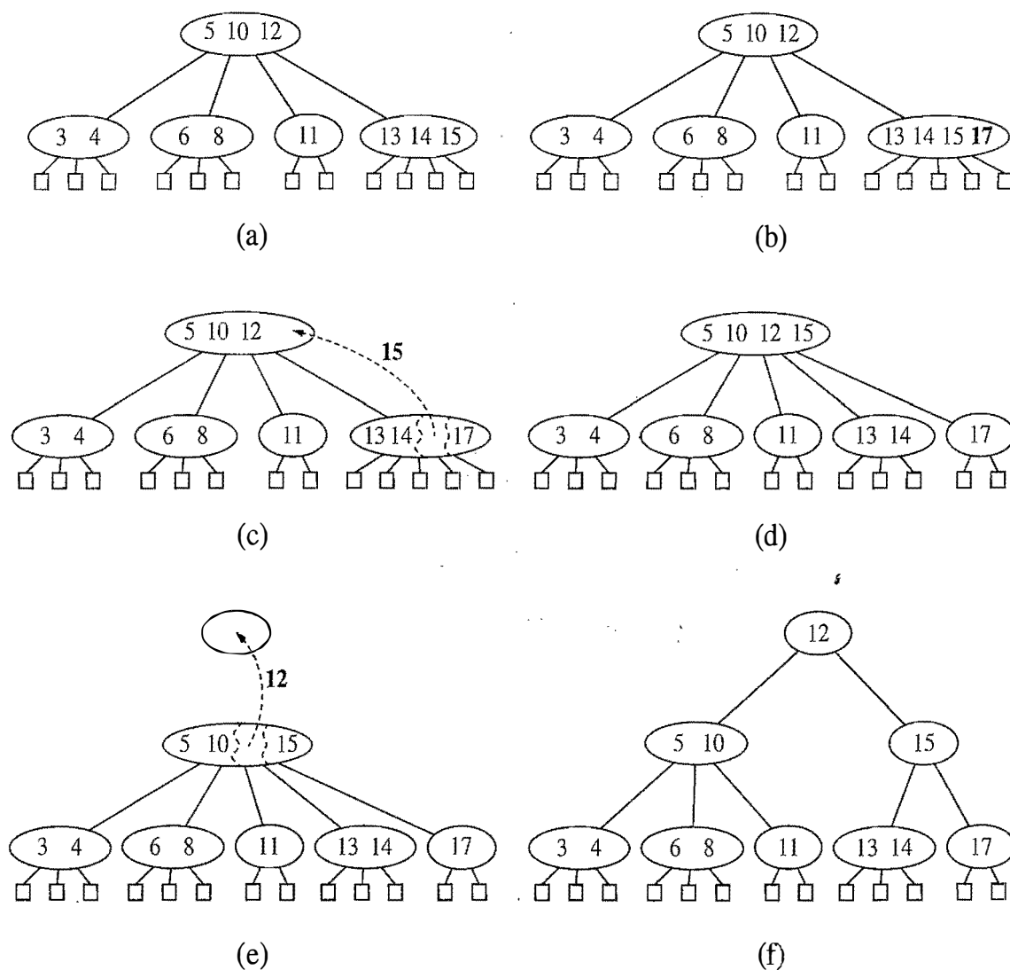
Figure 10.23: An insertion in a (2,4) tree that causes a cascading split: (a) before the insertion; (b) insertion of 17, causing an overflow; (c) a split; (d) after the split a new overflow occurs; (e) another split, creating a new root node; (f) final tree.
