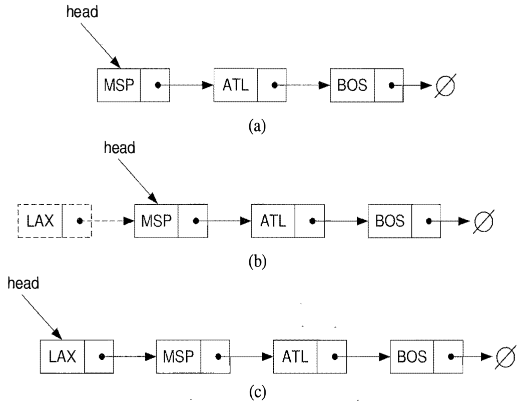
Figure 3.11: Insertion of an element at the head of a singly linked list: (a) before the insertion; (b) creation of a new node; (c) after the insertion.
