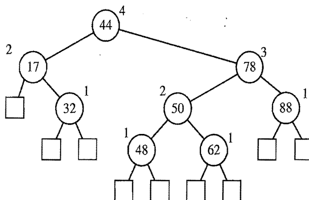
Figure 10.7: An example of an AVL tree. The keys of the entries are shown inside the nodes, and the heights of the nodes are shown next to the nodes.
