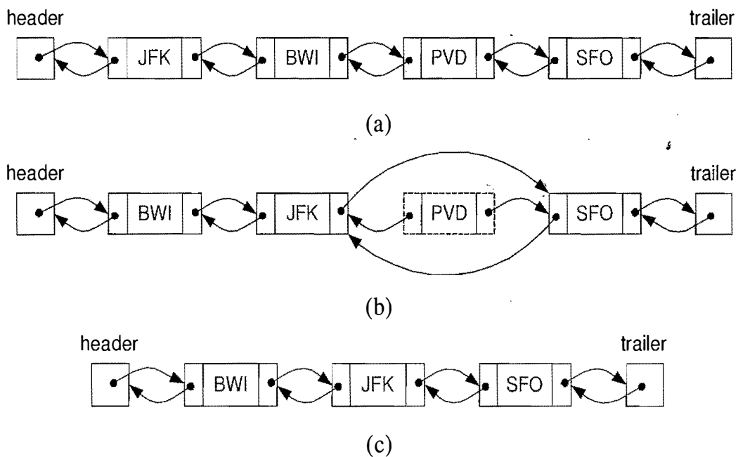
Figure 6.7: Removing the object stored at the position for “PVD”: (a) before the removal; (b) linking out the old node; (c) after the removal (and garbage collection).
