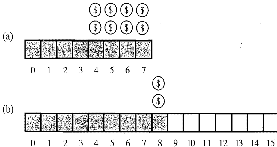
Figure 6.4: Illustration of a series of push operations on an array list: (a) an 8-cell array is full, with two cyber-rupees “stored” at cells 4 through 7; (b) a push operation causes an overflow and a doubling of capacity. Copying the eight old elements to the new array is paid for by the cyber-rupees already stored in the table. Inserting the new element is paid for by one of the cyber-rupees charged to the push operation, and the two cyber-rupees profited are stored at cell 8.
