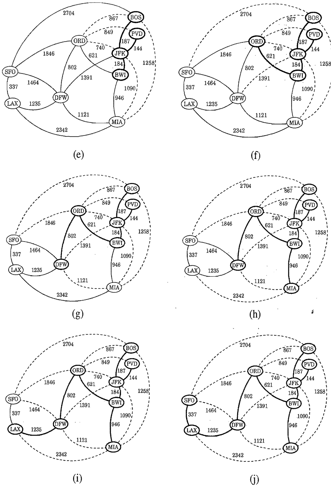
Figure 13.22: An illustration of the Prim-Jarník MST algorithm. (Continued from Figure 13.21.)
