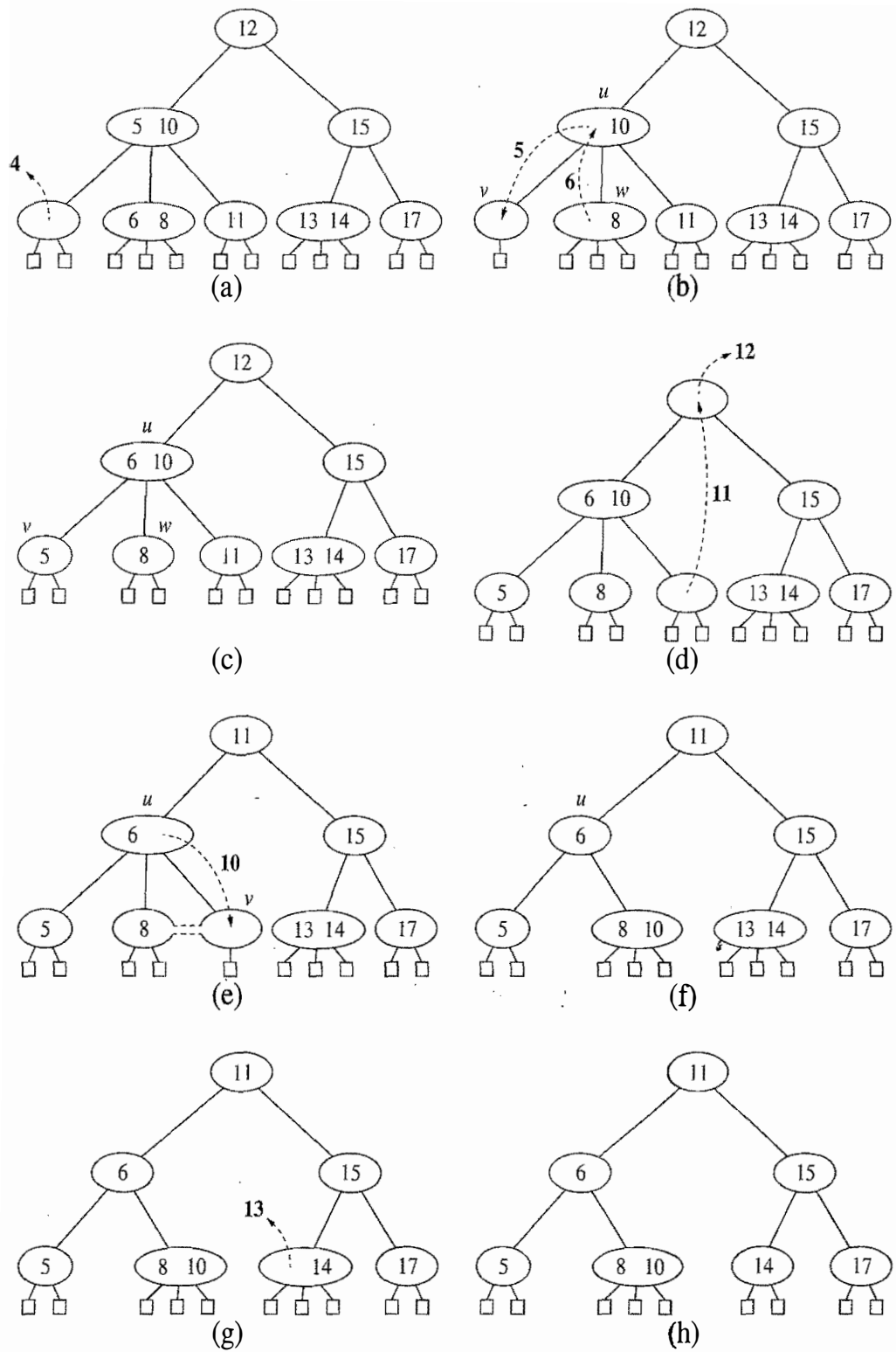
Figure 10.24: A sequence of removals from a (2,4) tree: (a) removal of 4, causing an underflow; (b) a transfer operation; (c) after the transfer operation; (d) removal of 12, causing an underflow; (e) a fusion operation; (f) after the fusion operation; (g) removal of 13; (h) after removing 13.
