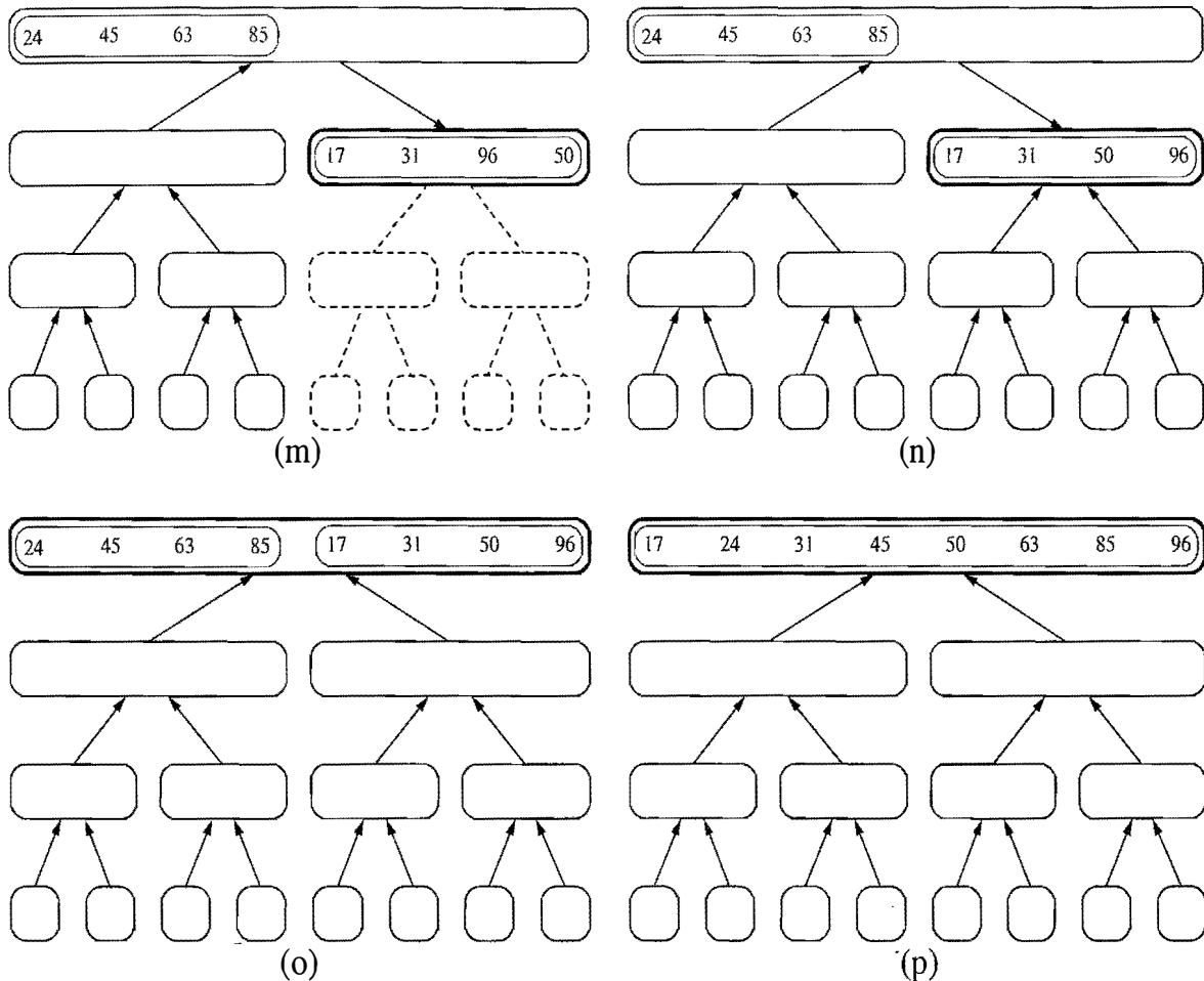
Figure 11.4: Visualization of an execution of merge-sort. Several invocations are omitted between (l) and (m) and between (m) and (n). Note the conquer step performed in step (p). (Continued from Figure 11.3.)
