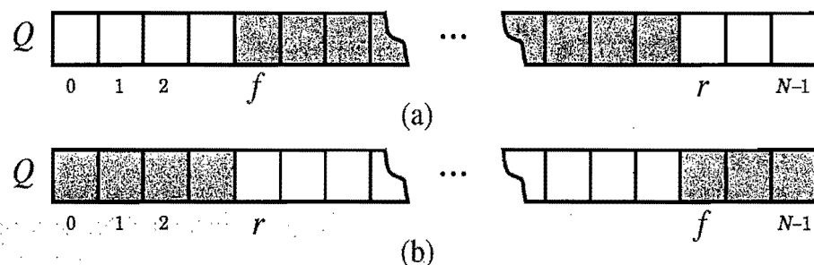
Figure 5.4: Using array Q in a circular fashion: (a) the “normal” configuration with f \leq r ; (b) the “wrapped around” configuration with r < f .
