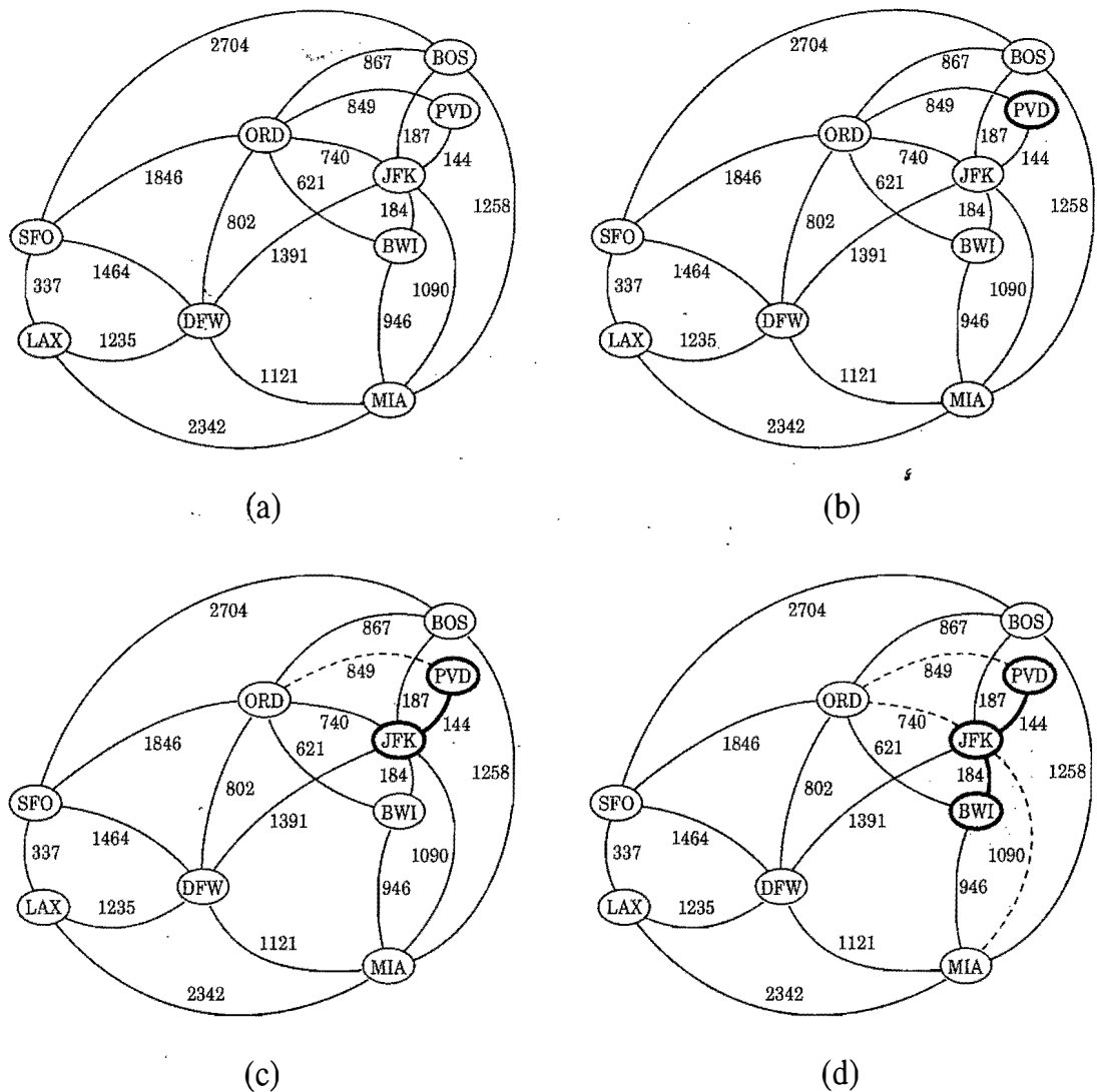
Figure 13.21: An illustration of the Prim-Jarník MST algorithm. (Continues in Figure 13.22.)
