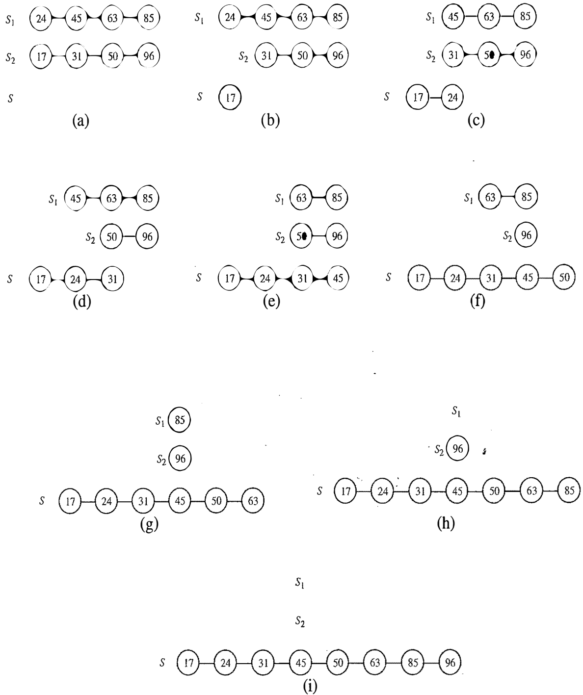
Figure 11.6: Example of an execution of the algorithm merge shown in Code Fragment 11.2.
