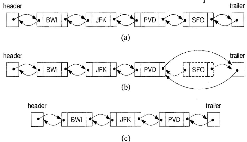
Figure 3.15: Removing the node at the end of a doubly linked list with header and trailer sentinels: (a) before deleting at the tail; (b) deleting at the tail; (c) after the deletion.
