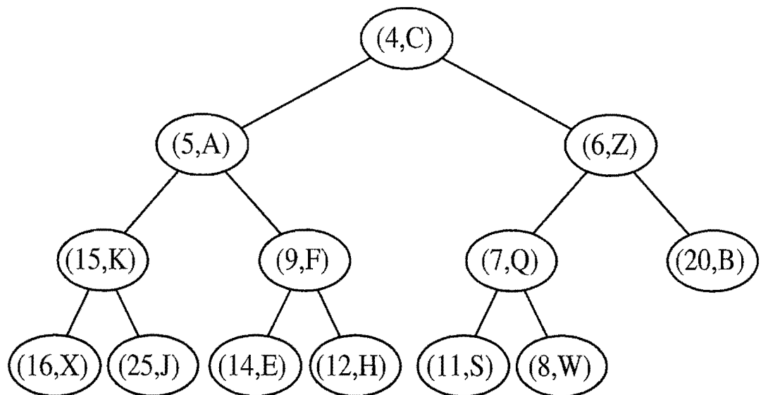
Figure 8.3: Example of a heap storing 13 entries with integer keys. The last node is the one storing entry (8, W) .
