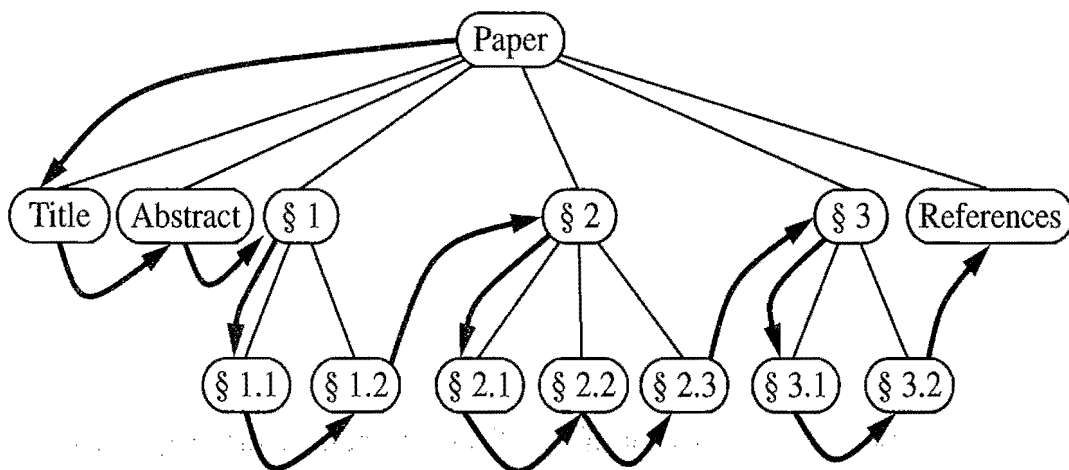
Figure 7.6: Preorder traversal of an ordered tree, where the children of each node are ordered from left to right.
