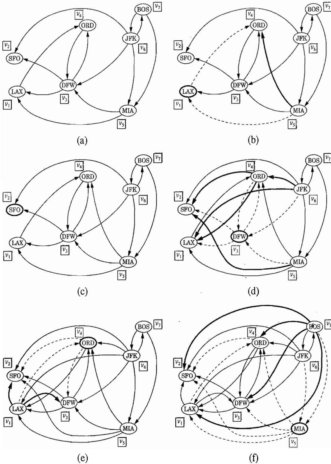
Figure 13.10: Sequence of digraphs computed by the Floyd-Warshall algorithm: (a) initial digraph \vec{G} = \vec{G}_0 and numbering of the vertices; (b) digraph \vec{G}_1 ; (c) \vec{G}_2 ; (d) \vec{G}_3 ; (e) \vec{G}_4 ; (f) \vec{G}_5 . Note that \vec{G}_5 = \vec{G}_6 = \vec{G}_7 . If digraph \vec{G}_{k-1} has the edges (v_i, v_k) and (v_k, v_j) , but not the edge (v_i, v_j) , in the drawing of digraph \vec{G}_k , we show edges (v_i, v_k) and (v_k, v_j) with dashed blue lines, and edge (v_i, v_j) with a thick blue line.
