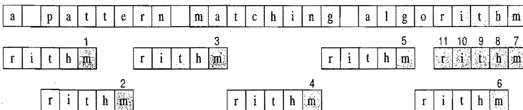
Figure 12.6: An example of a Boyer-Moore execution on English text.
