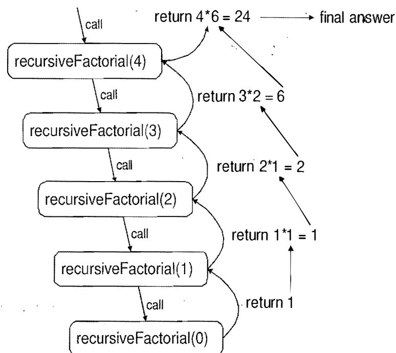
Figure 3.21: A recursion trace for the call recursiveFactorial(4) .
