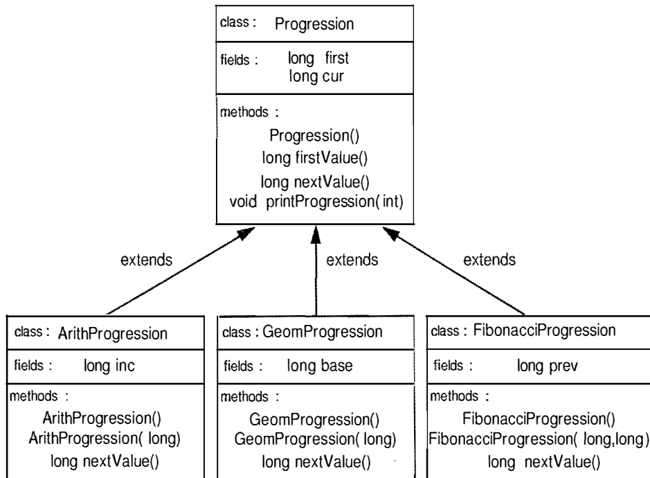
Figure 2.5: Inheritance diagram for class Progression and its subclasses.
