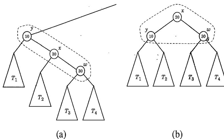
Figure 10.14: Zig: (a) before; (b) after. There is another symmetric configuration where x and w are left children.
