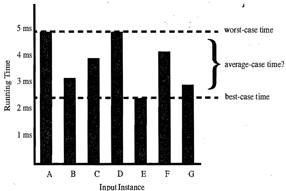
Figure 4.4: The difference between best-case and worst-case time. Each bar represents the running time of some algorithm on a different possible input.
