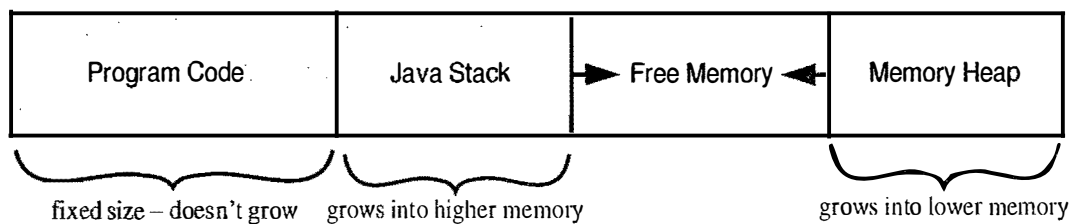
Figure 14.2: A schematic view of the layout of memory addresses in the Java Virtual Machine.
