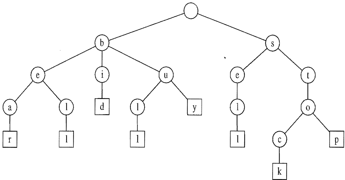
Figure 12.9: Standard trie for the strings {bear, bell, bid, bull, buy, sell, stock, stop}.
