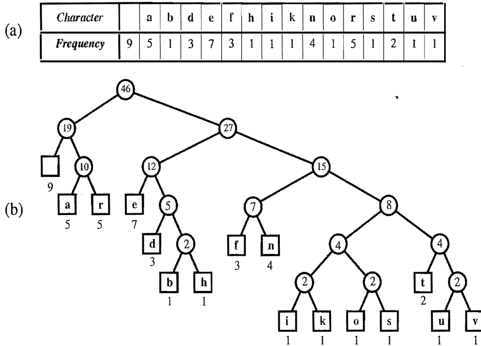
Figure 12.8: An illustration of an example Huffman code for the input string X = \text{"a fast runner need never be afraid of the dark"} : (a) frequency of each character of X ; (b) Huffman tree T for string X . The code for a character c is obtained by tracing the path from the root of T to the external node where c is stored, and associating a left child with 0 and a right child with 1. For example, the code for “a” is 010, and the code for “f” is 1100.
