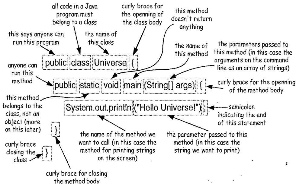
Figure 1.1: A “Hello Universe!” program.
