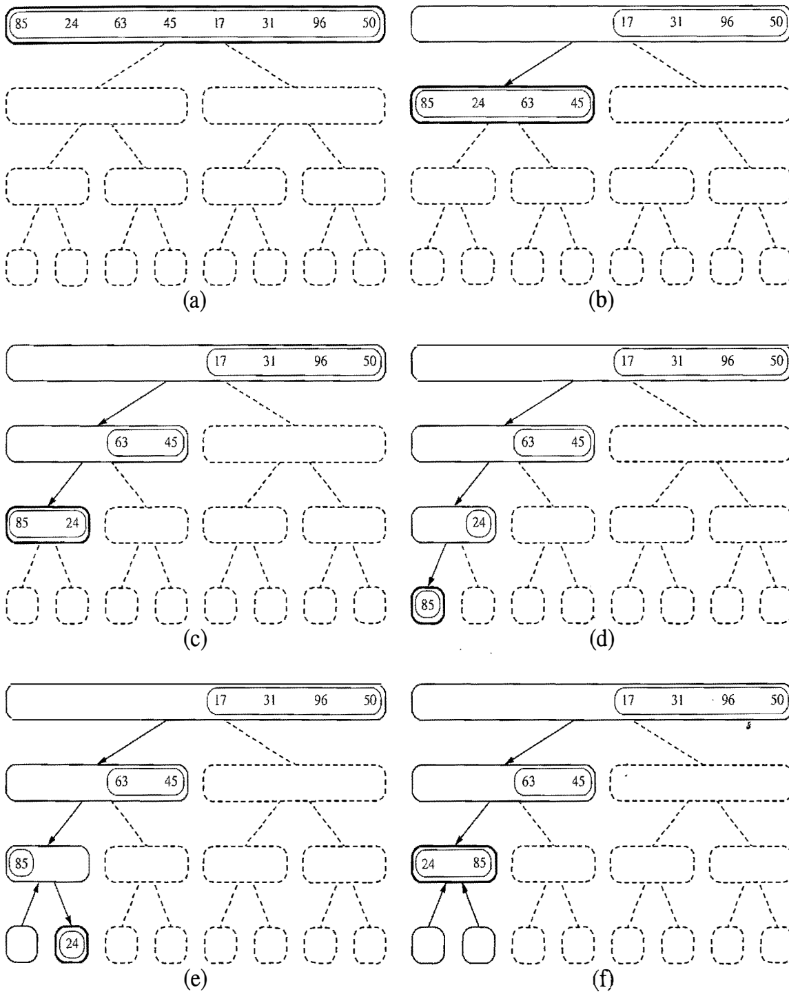
Figure 11.2: Visualization of an execution of merge-sort. Each node of the tree represents a recursive call of merge-sort. The nodes drawn with dashed lines represent calls that have not been made yet. The node drawn with thick lines represents the current call. The empty nodes drawn with thin lines represent completed calls. The remaining nodes (drawn with thin lines and not empty) represent calls that are waiting for a child invocation to return. (Continues in Figure 11.3.)
