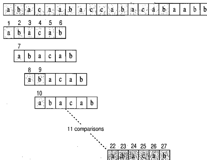
Figure 12.3: Example run of the brute-force pattern matching algorithm. The algorithm performs 27 character comparisons, indicated above with numerical labels.
