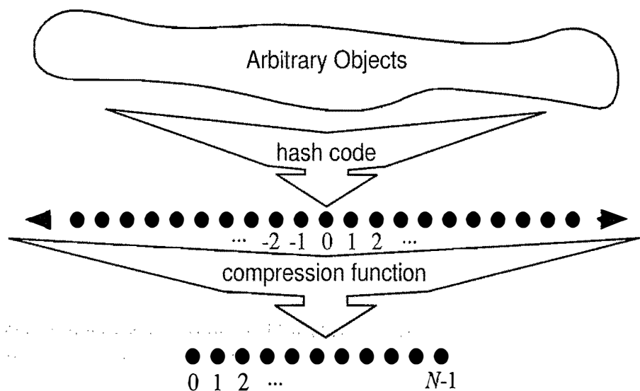
Figure 9.3: The two parts of a hash function: a hash code and a compression function.
