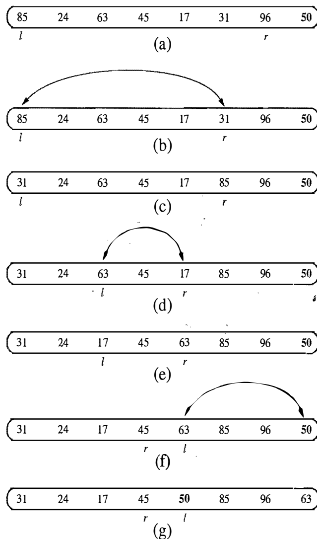
Figure 11.14: Divide step of in-place quick-sort. Index l scans the sequence from left to right, and index r scans the sequence from right to left. A swap is performed when l is at an element larger than the pivot and r is at an element smaller than the pivot. A final swap with the pivot completes the divide step.
