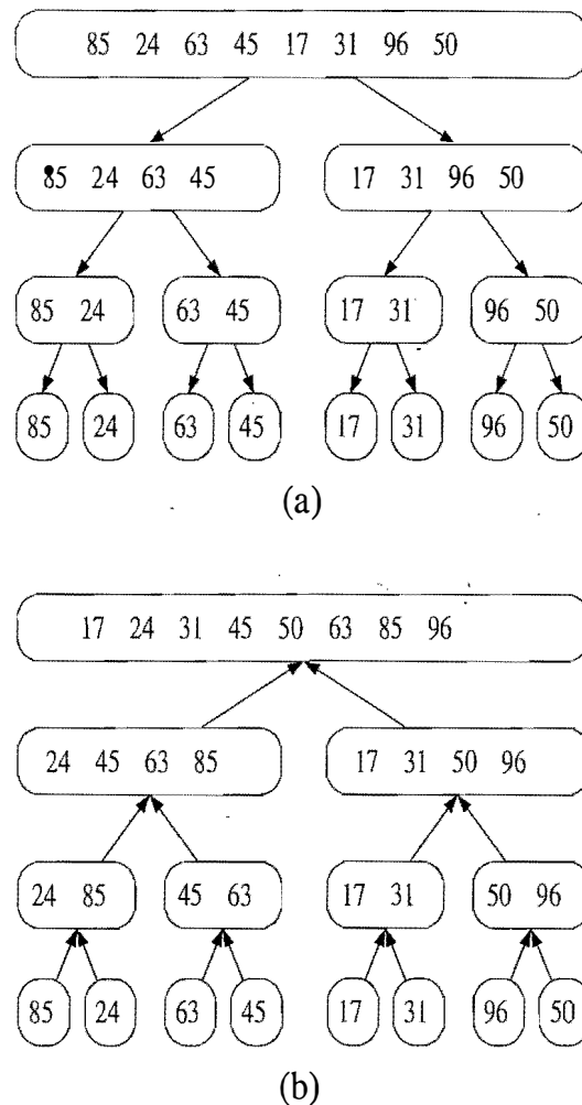
Figure 11.1: Merge-sort tree T for an execution of the merge-sort algorithm on a sequence with 8 elements: (a) input sequences processed at each node of T ; (b) output sequences generated at each node of T .
