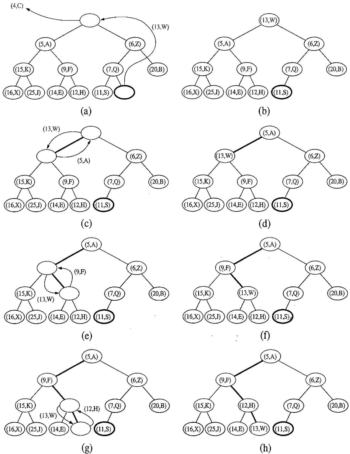
Figure 8.8: Removal of the entry with the smallest key from a heap: (a and b) deletion of the last node, whose entry gets stored into the root; (c and d) swap to locally restore the heap-order property; (e and f) another swap; (g and h) final swap.
