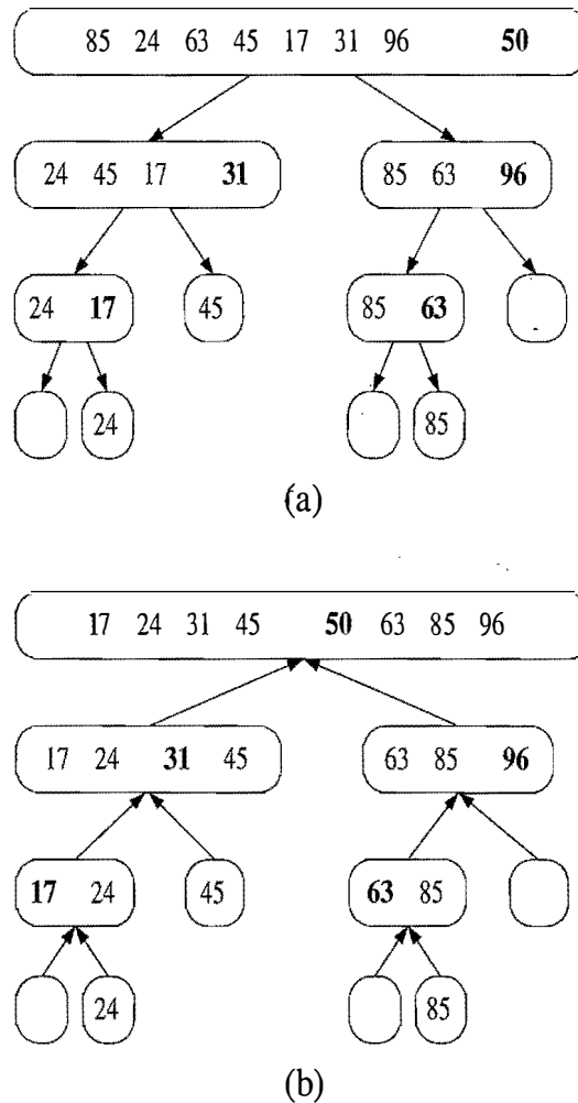
Figure 11.9: Quick-sort tree T for an execution of the quick-sort algorithm on a sequence with 8 elements: (a) input sequences processed at each node of T ; (b) output sequences generated at each node of T . The pivot used at each level of the recursion is shown in bold.
