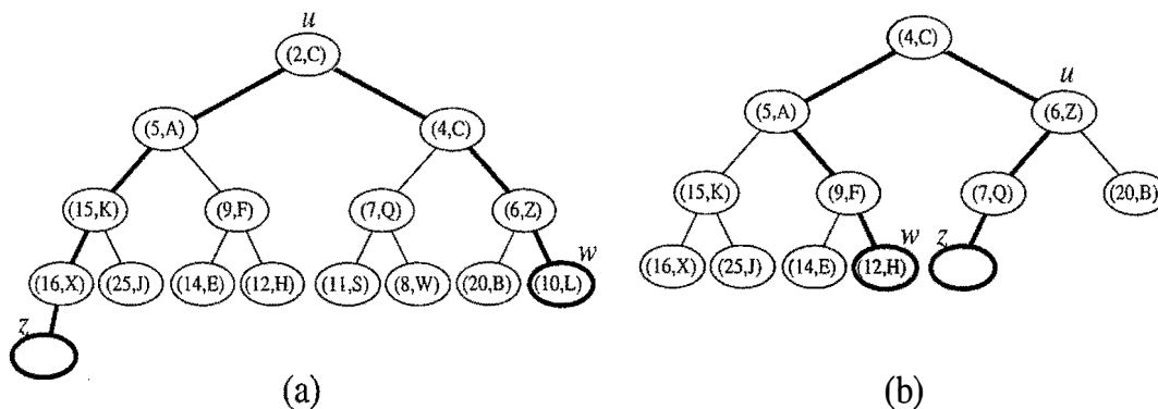
Figure 8.12: Updating the last node in a complete binary tree after operation add or remove. Node w is the last node before operation add or after operation remove. Node z is the last node after operation add or before operation remove.
