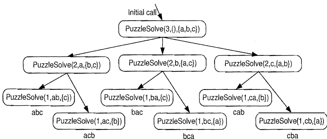
Figure 3.26: Recursion trace for an execution of \text{PuzzleSolve}(3, S, U) , where S is empty and U = \{a, b, c\} . This execution generates and tests all permutations of a , b , and c . We show the permutations generated directly below their respective boxes.
