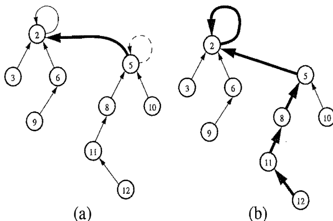
Figure 11.18: Tree-based implementation of a partition: (a) operation \text{union}(A, B) ; (b) operation \text{find}(p) , where p denotes the position object for element 12.
