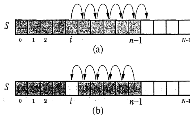
Figure 6.1: Array-based implementation of an array list S that is storing n elements: (a) shifting up for an insertion at index i ; (b) shifting down for a removal at index i .
