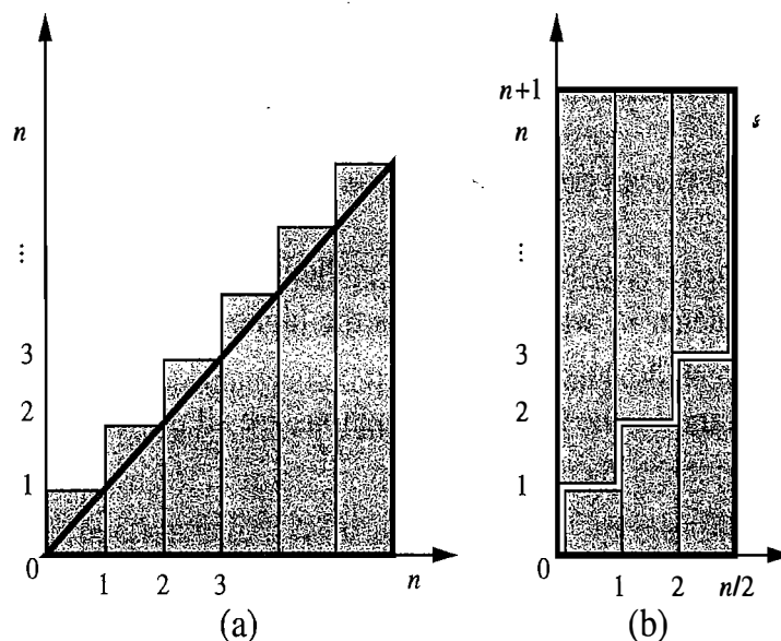
Figure 4.1: Visual justifications of Proposition 4.3. Both illustrations visualize the identity in terms of the total area covered by n unit-width rectangles with heights 1, 2, \dots, n . In (a) the rectangles are shown to cover a big triangle of area n^2/2 (base n and height n ) plus n small triangles of area 1/2 each (base 1 and height 1). In (b), which applies only when n is even, the rectangles are shown to cover a big rectangle of base n/2 and height n + 1 .
