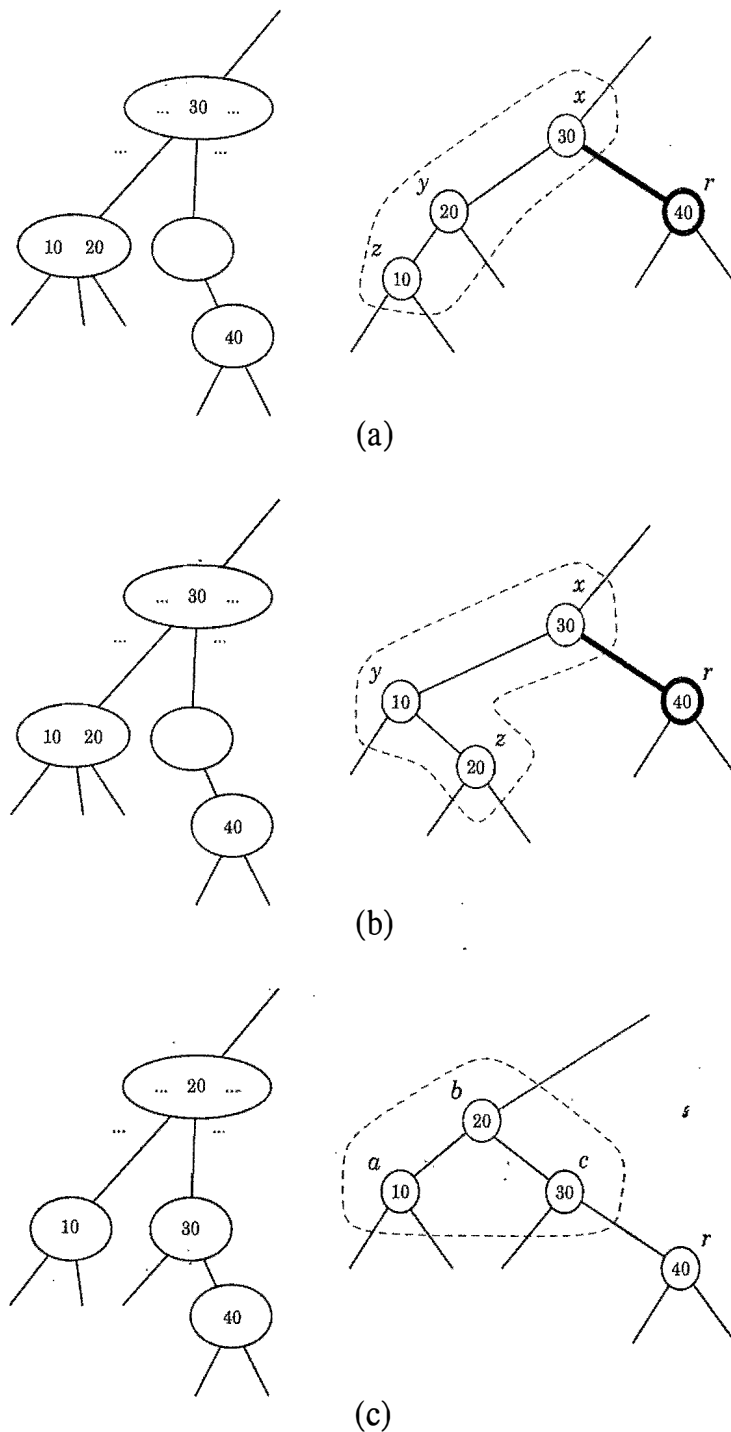
Figure 10.32: Restructuring of a red-black tree to remedy the double black problem: (a) and (b) configurations before the restructuring, where r is a right child and the associated nodes in the corresponding (2,4) tree before the transfer (two other symmetric configurations where r is a left child are possible); (c) configuration after the restructuring and the associated nodes in the corresponding (2,4) tree after the transfer. The grey color for node x in parts (a) and (b) and for node b in part (c) denotes the fact that this node may be colored either red or black.
