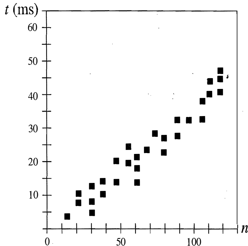
Figure 4.3: Results of an experimental study on the running time of an algorithm. A dot with coordinates (n, t) indicates that on an input of size n , the running time of the algorithm is t milliseconds (ms).
