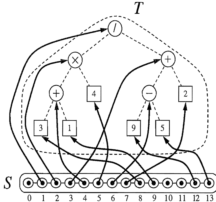
Figure 7.16: Representation of a binary tree T by means of an array list S .
