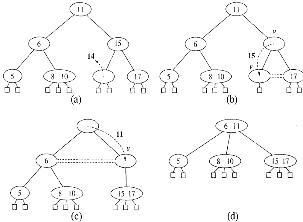
Figure 10.25: A propagating sequence of fusions in a (2,4) tree: (a) removal of 14, which causes an underflow; (b) fusion, which causes another underflow; (c) second fusion operation, which causes the root to be removed; (d) final tree.
