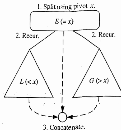
Figure 11.8: A visual schematic of the quick-sort algorithm.
