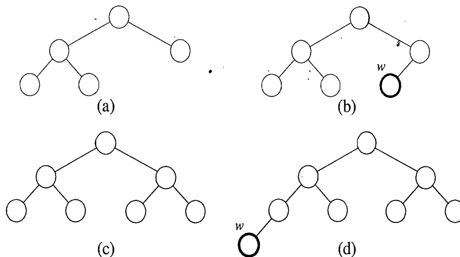
Figure 8.4: Examples of operations add and remove on a complete binary tree, where w denotes the node inserted by add or deleted by remove. The trees shown in (b) and (d) are the results of performing add operations on the trees in (a) and (c), respectively. Likewise, the trees shown in (a) and (c) are the results of performing remove operations on the trees in (b) and (d), respectively.
