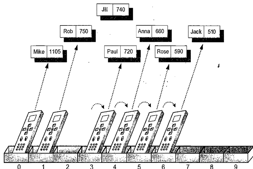
Figure 3.2: Preparing to add a new GameEntry object to the entries array. In order to make room for the new reference, we have to shift the references to game entries with smaller scores than the new one to the right by one cell.
