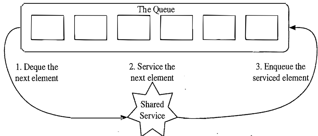
Figure 5.5: The three iterative steps for using a queue to implement a round robin scheduler.
