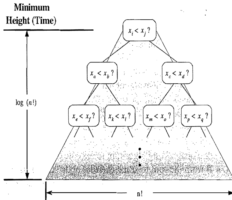
Figure 11.15: Visualizing the lower bound for comparison-based sorting.
