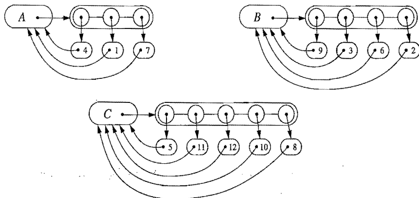
Figure 11.16: Sequence-based implementation of a partition consisting of three sets: A = \{1, 4, 7\} , B = \{2, 3, 6, 9\} , and C = \{5, 8, 10, 11, 12\} .
