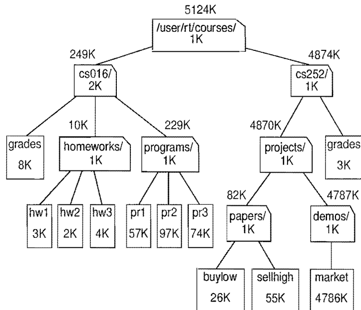
Figure 7.9: The tree of Figure 7.3 representing a file system, showing the name and size of the associated file/directory inside each node, and the disk space used by the associated directory above each internal node.
