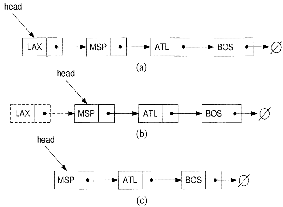
Figure 3.13: Removal of an element at the head of a singly linked list: (a) before the removal; (b) “linking out” the old new node; (c) after the removal.
