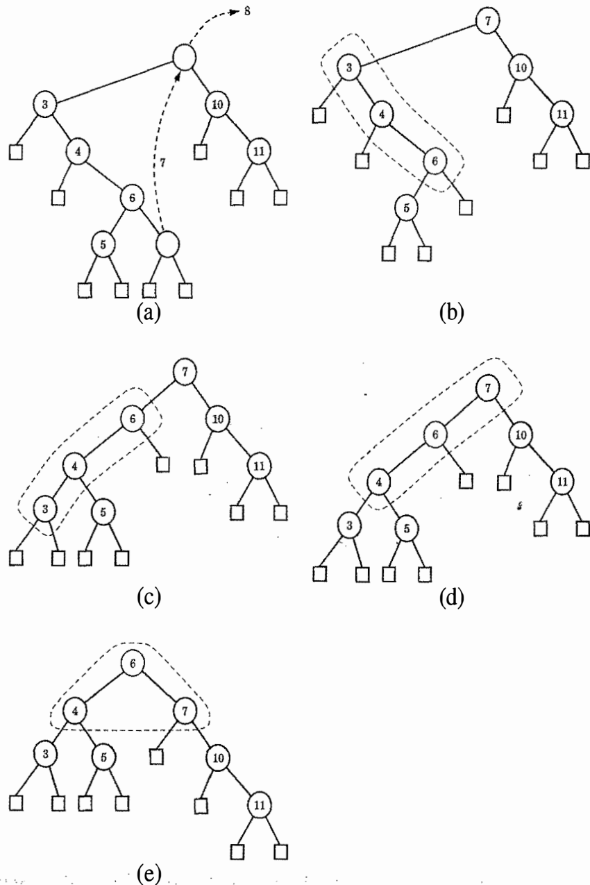
Figure 10.18: Deletion from a splay tree: (a) the deletion of 8 from node r is performed by moving to r the key of the right-most internal node v , in the left subtree of r , deleting v , and splaying the parent u of v ; (b) splaying u starts with a zig-zig; (c) after the zig-zig; (d) the next step is a zig; (e) after the zig.
