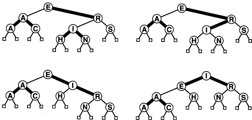
Figure 15.12 Splitting a node in a red-black tree.
