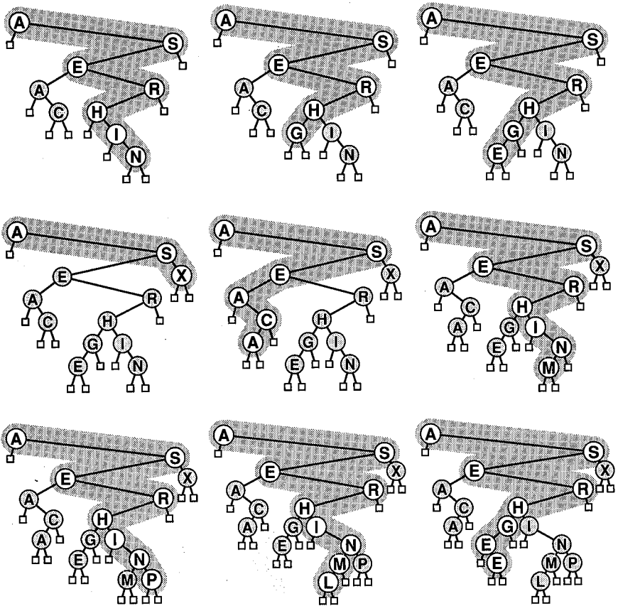
Figure 14.10 Building a binary search tree.
