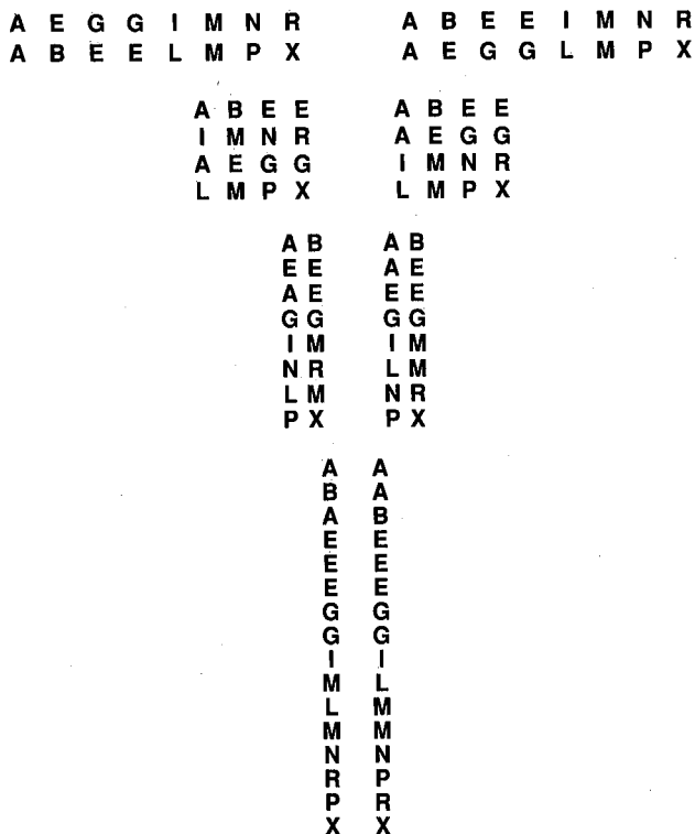
Figure 40.2 Split-and-interleave merging.
