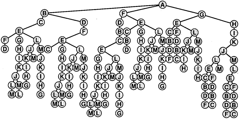
Figure 44.2 Exhaustive search.
