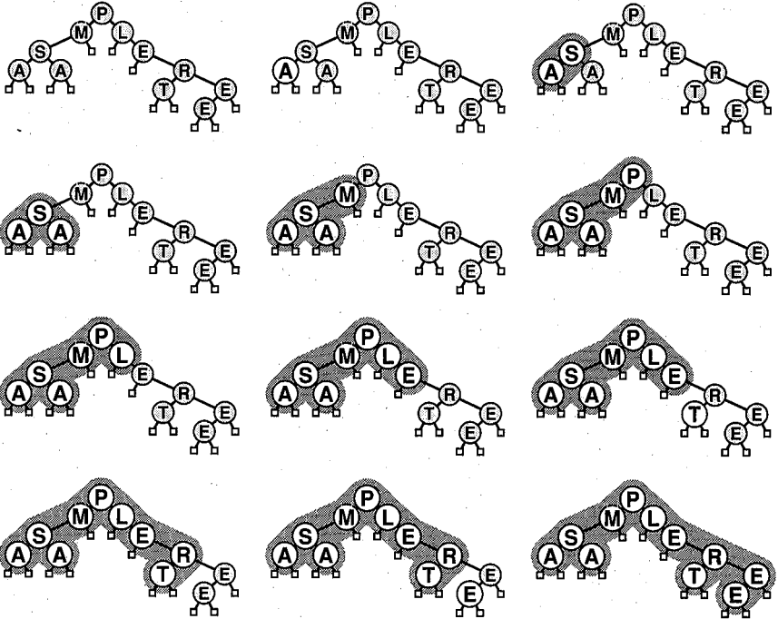
Figure 4.10 Inorder traversal.
