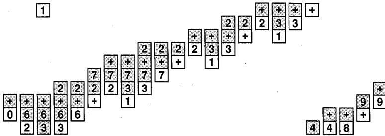
Figure 20.8 Contents of deque during recognition of AAABD.
