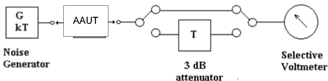
Figure 2: Measurement arrangement
