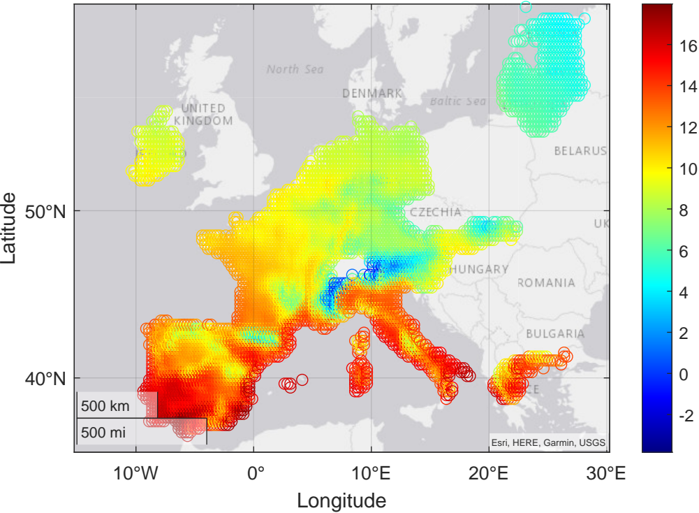
Historical Mean Surface for 50-80s
