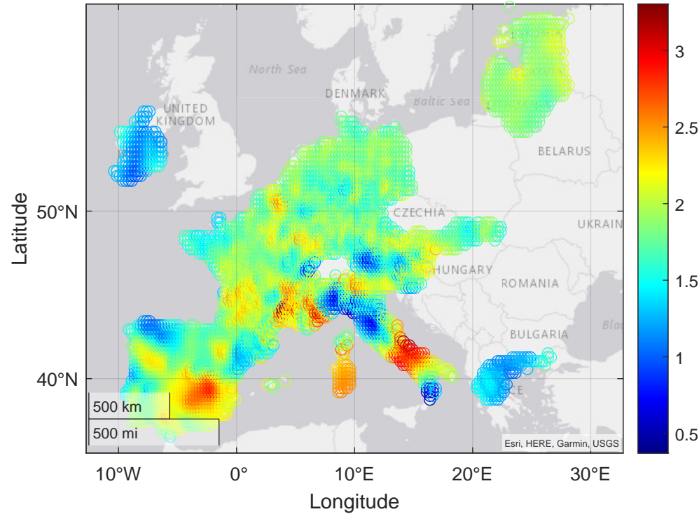
Deviation from the Mean Surface in 2001-2021
